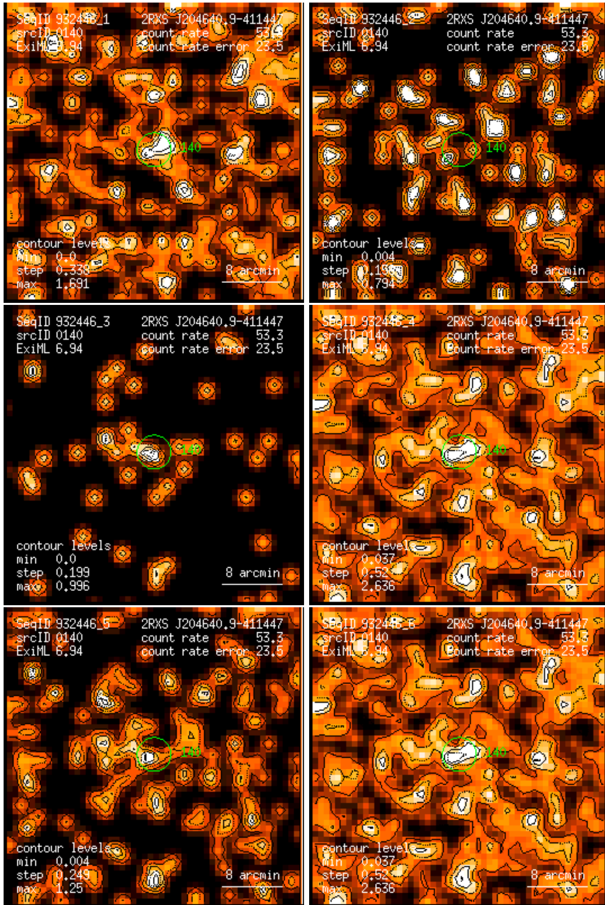
Figure 140: RASS 932446: detection 0140: band rate images, Gaussian filter: (1) PSPC channels 11 – 41, (2) 52 – 90, (3) 91 – 201, (4) 11 – 235, (5) 52 – 201, (6) 11 – 201. Broad band rates in counts/ks. Band rate contour levels in counts/ks/arcmin 2 .
