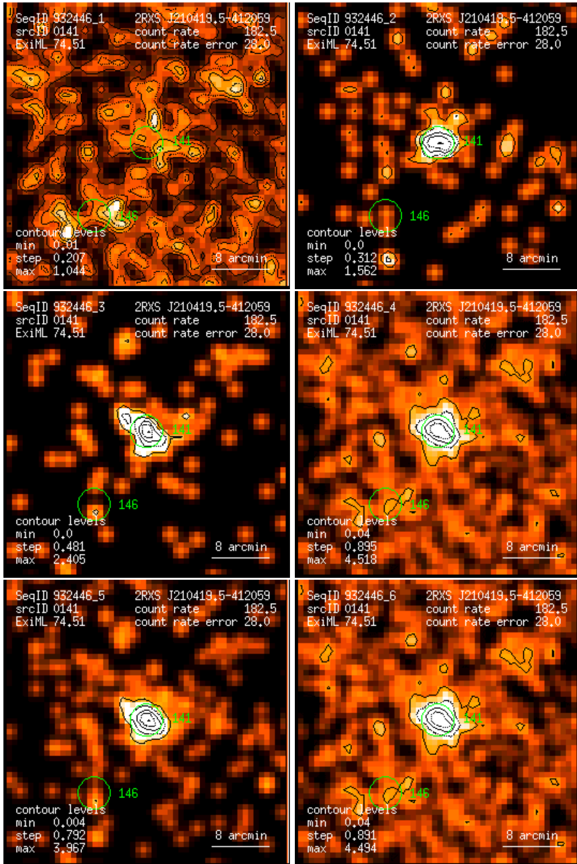
Figure 141: RASS 932446: detection 0141: band rate images, Gaussian filter: (1) PSPC channels 11 – 41, (2) 52 – 90, (3) 91 – 201, (4) 11 – 235, (5) 52 – 201, (6) 11 – 201. Broad band rates in counts/ks. Band rate contour levels in counts/ks/arcmin 2 .
