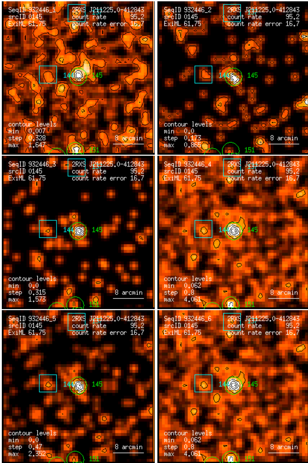
Figure 145: RASS 932446: detection 0145: band rate images, Gaussian filter: (1) PSPC channels 11 – 41, (2) 52 – 90, (3) 91 – 201, (4) 11 – 235, (5) 52 – 201, (6) 11 – 201. Broad band rates in counts/ks. Band rate contour levels in counts/ks/arcmin 2 .
