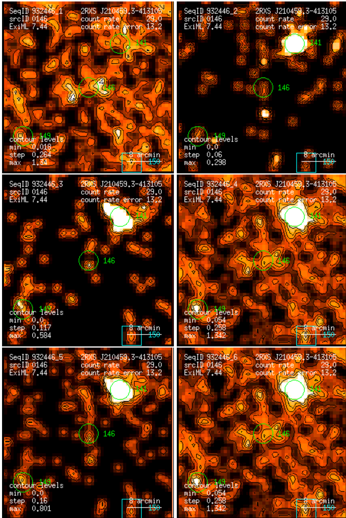
Figure 146: RASS 932446: detection 0146: band rate images, Gaussian filter: (1) PSPC channels 11 – 41, (2) 52 – 90, (3) 91 – 201, (4) 11 – 235, (5) 52 – 201, (6) 11 – 201. Broad band rates in counts/ks. Band rate contour levels in counts/ks/arcmin 2 .
