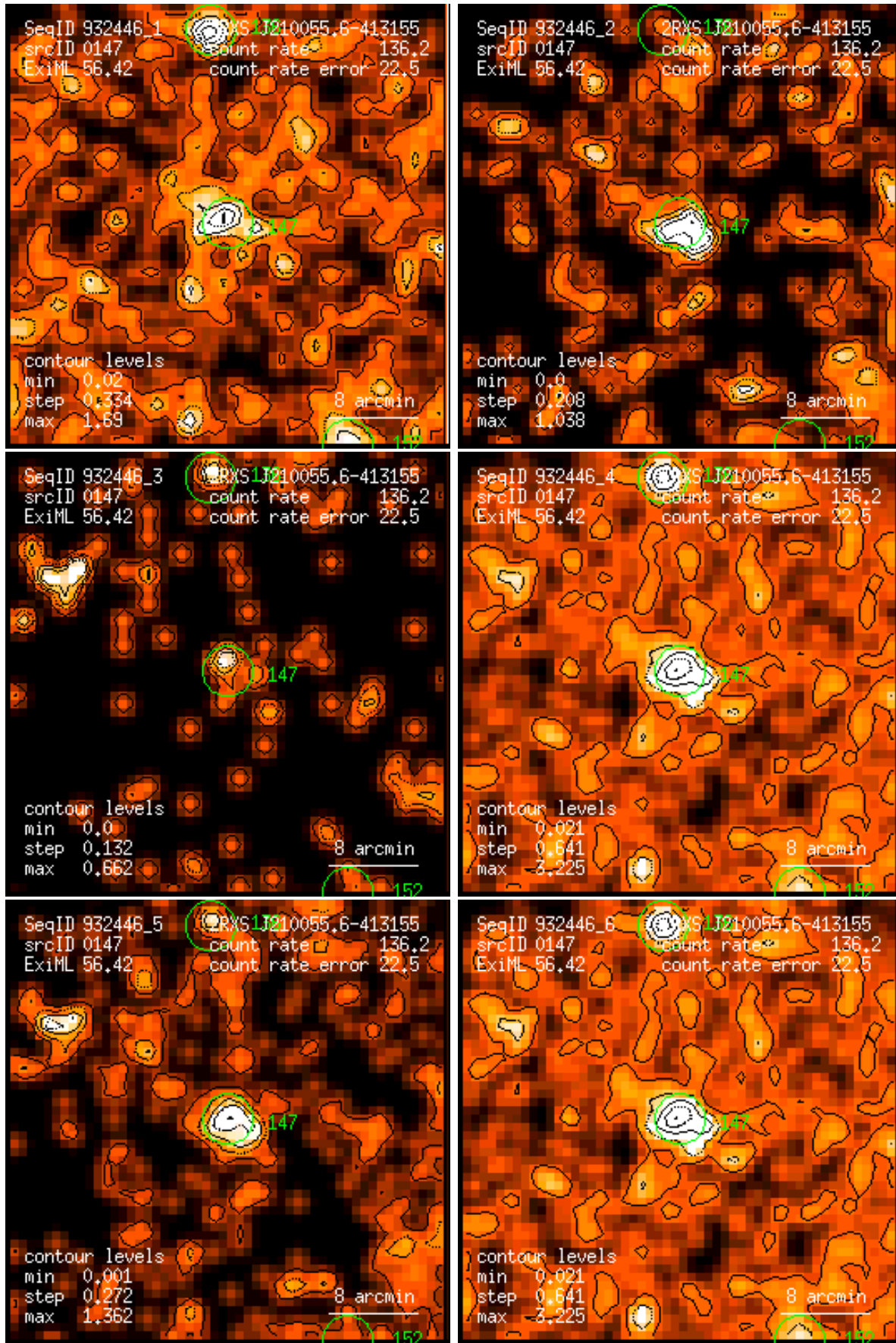
Figure 147: RASS 932446: detection 0147: band rate images, Gaussian filter: (1) PSPC channels 11 – 41, (2) 52 – 90, (3) 91 – 201, (4) 11 – 235, (5) 52 – 201, (6) 11 – 201. Broad band rates in counts/ks. Band rate contour levels in counts/ks/arcmin 2 .
