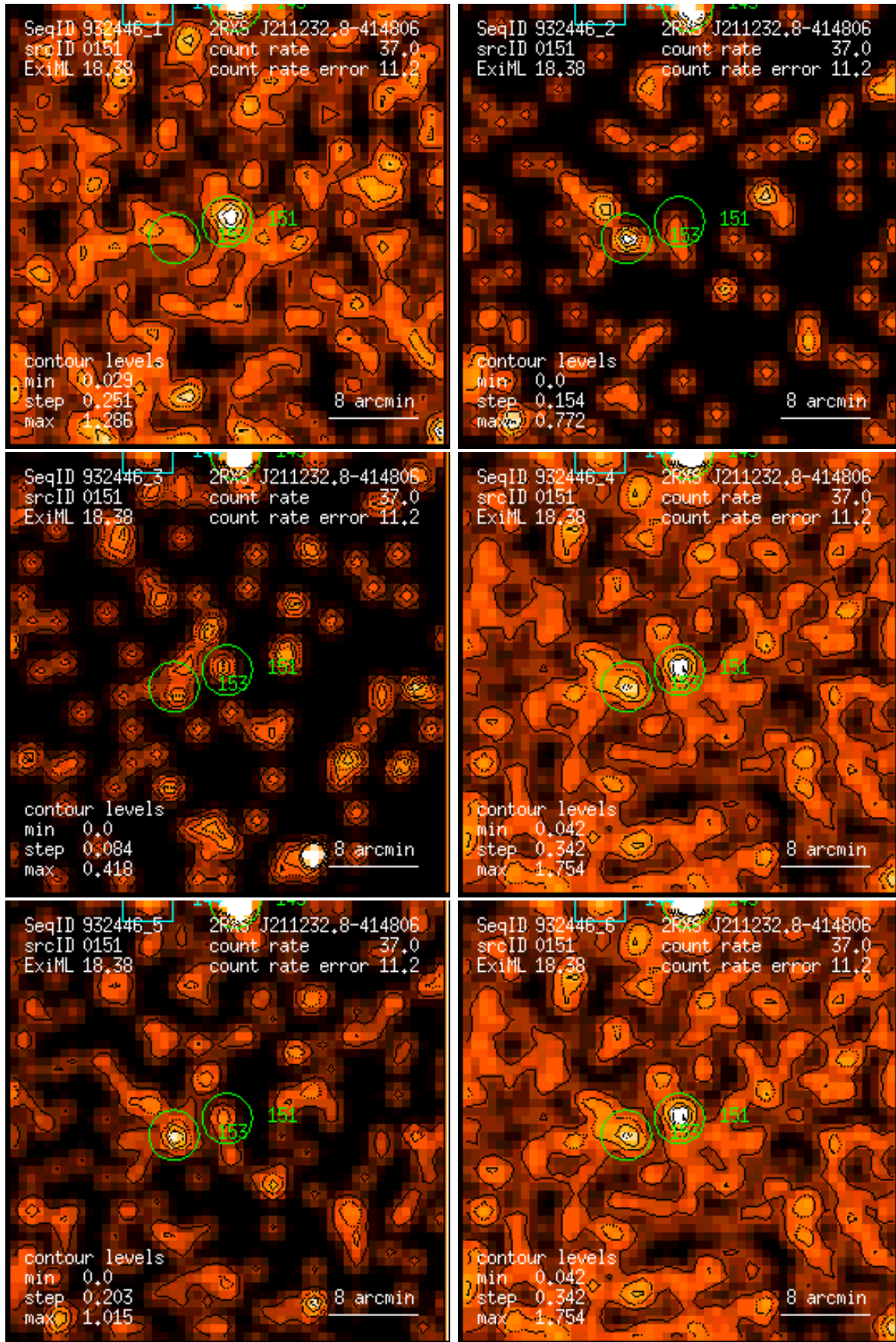
Figure 151: RASS 932446: detection 0151: band rate images, Gaussian filter: (1) PSPC channels 11 – 41, (2) 52 – 90, (3) 91 – 201, (4) 11 – 235, (5) 52 – 201, (6) 11 – 201. Broad band rates in counts/ks. Band rate contour levels in counts/ks/arcmin 2 .
