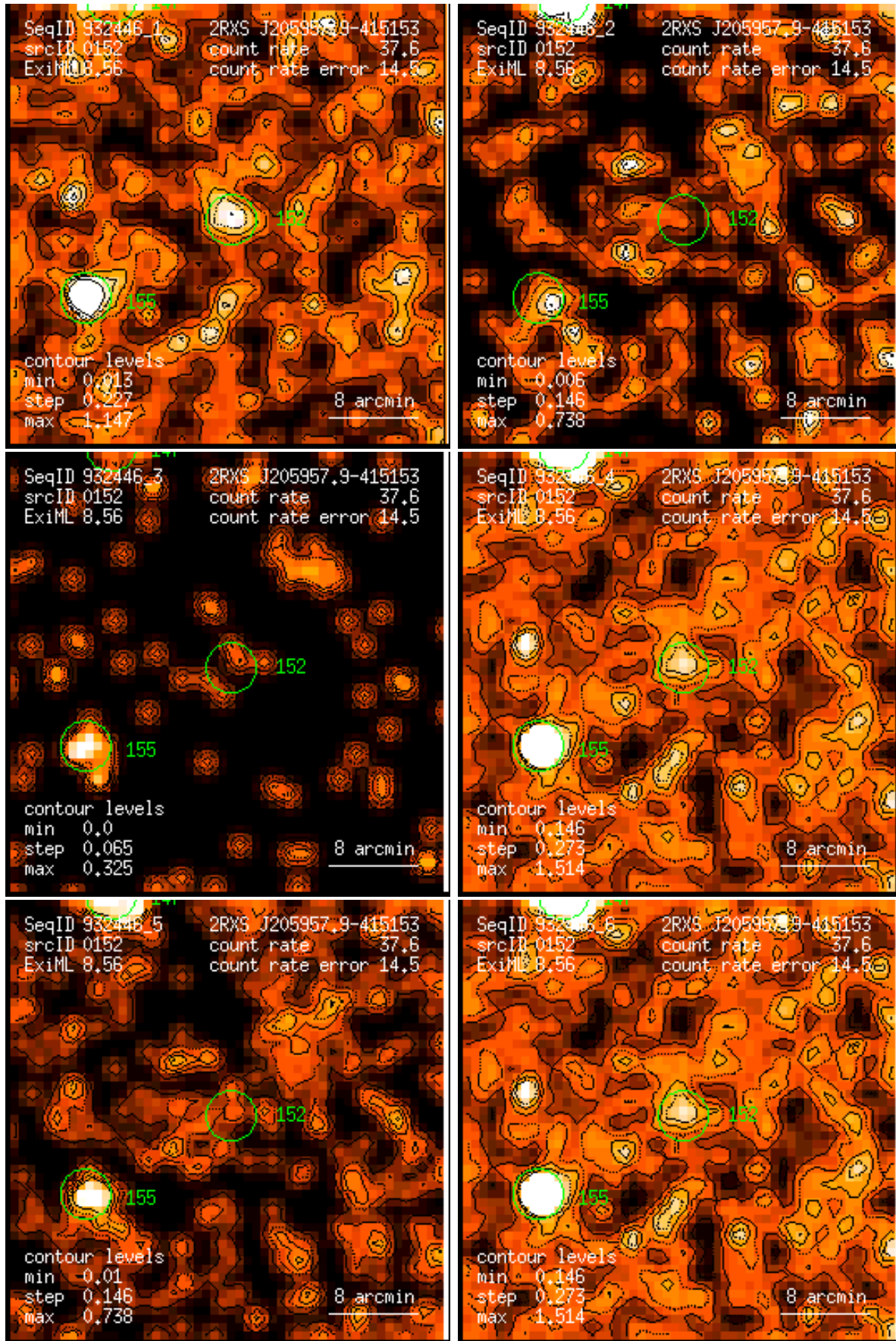
Figure 152: RASS 932446: detection 0152: band rate images, Gaussian filter: (1) PSPC channels 11 – 41, (2) 52 – 90, (3) 91 – 201, (4) 11 – 235, (5) 52 – 201, (6) 11 – 201. Broad band rates in counts/ks. Band rate contour levels in counts/ks/arcmin 2 .
