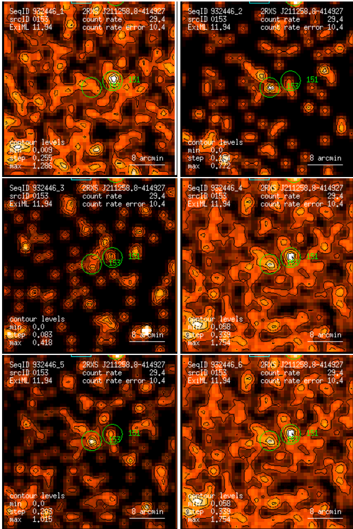
Figure 153: RASS 932446: detection 0153: band rate images, Gaussian filter: (1) PSPC channels 11 – 41, (2) 52 – 90, (3) 91 – 201, (4) 11 – 235, (5) 52 – 201, (6) 11 – 201. Broad band rates in counts/ks. Band rate contour levels in counts/ks/arcmin 2 .
