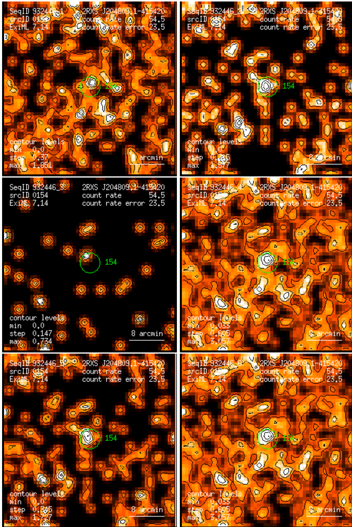
Figure 154: RASS 932446: detection 0154: band rate images, Gaussian filter: (1) PSPC channels 11 – 41, (2) 52 – 90, (3) 91 – 201, (4) 11 – 235, (5) 52 – 201, (6) 11 – 201. Broad band rates in counts/ks. Band rate contour levels in counts/ks/arcmin 2 .
