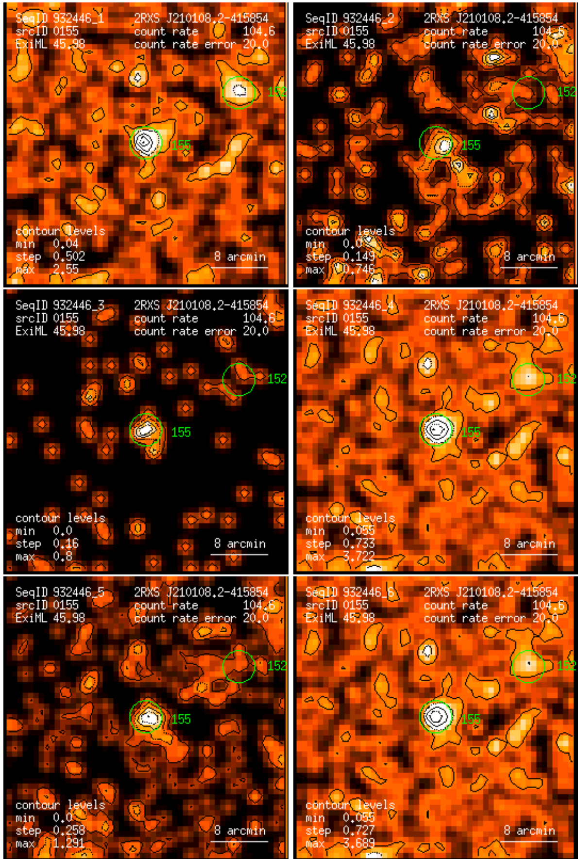
Figure 155: RASS 932446: detection 0155: band rate images, Gaussian filter: (1) PSPC channels 11 – 41, (2) 52 – 90, (3) 91 – 201, (4) 11 – 235, (5) 52 – 201, (6) 11 – 201. Broad band rates in counts/ks. Band rate contour levels in counts/ks/arcmin 2 .
