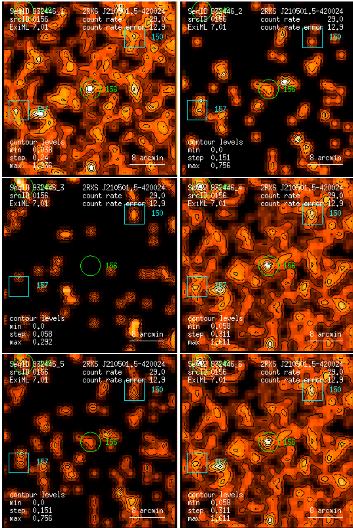
Figure 156: RASS 932446: detection 0156: band rate images, Gaussian filter: (1) PSPC channels 11 – 41, (2) 52 – 90, (3) 91 – 201, (4) 11 – 235, (5) 52 – 201, (6) 11 – 201. Broad band rates in counts/ks. Band rate contour levels in counts/ks/arcmin 2 .
