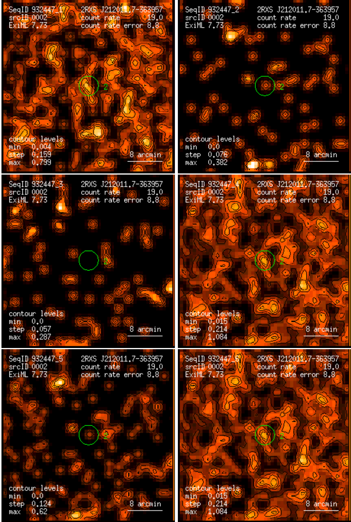
Figure 2: RASS 932447: detection 0002: band rate images, Gaussian filter: (1) PSPC channels 11 – 41, (2) 52 – 90, (3) 91 – 201, (4) 11 – 235, (5) 52 – 201, (6) 11 – 201. Broad band rates in counts/ks. Band rate contour levels in counts/ks/arcmin 2 .
