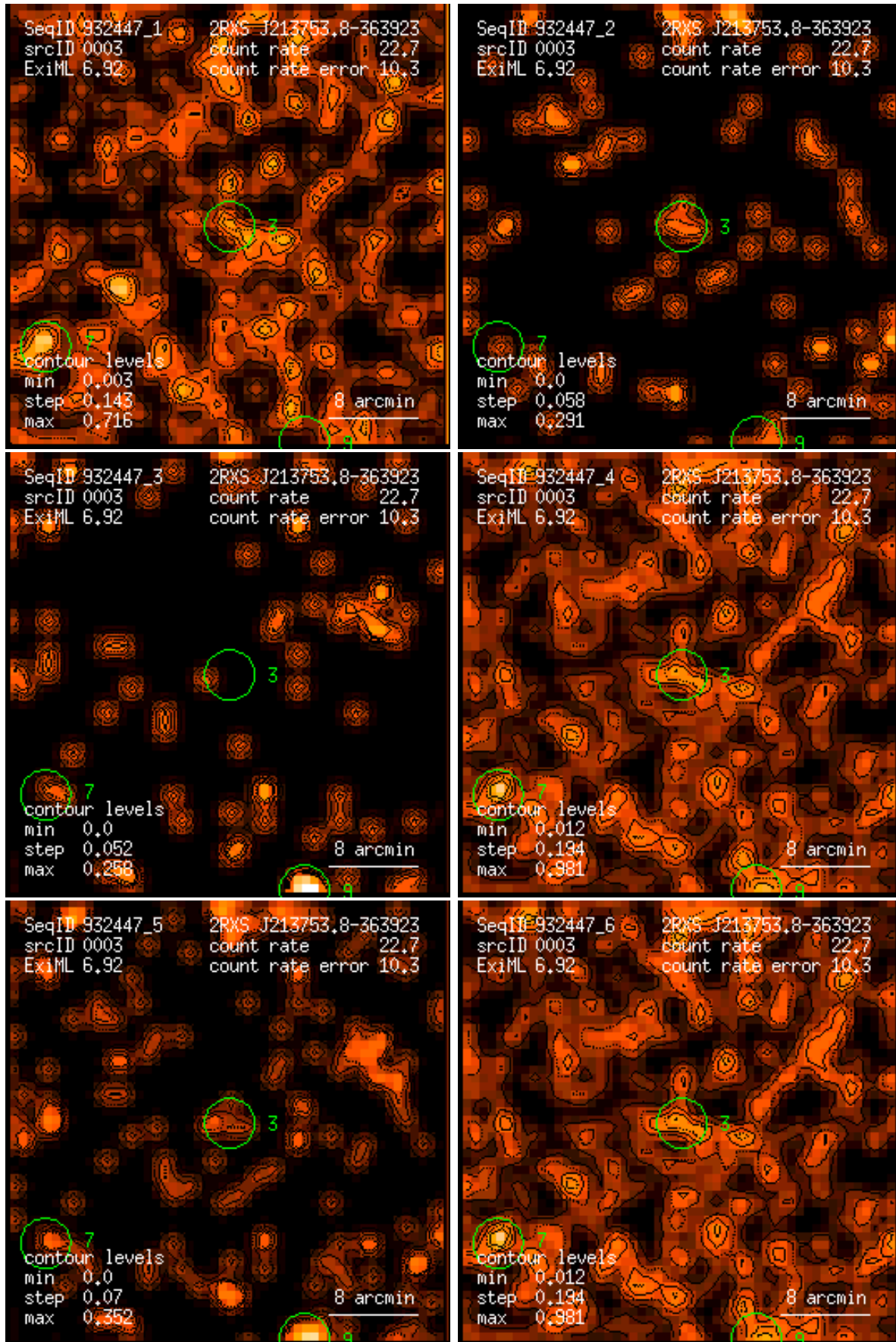
Figure 3: RASS 932447: detection 0003: band rate images, Gaussian filter: (1) PSPC channels 11 – 41, (2) 52 – 90, (3) 91 – 201, (4) 11 – 235, (5) 52 – 201, (6) 11 – 201. Broad band rates in counts/ks. Band rate contour levels in counts/ks/arcmin 2 .
