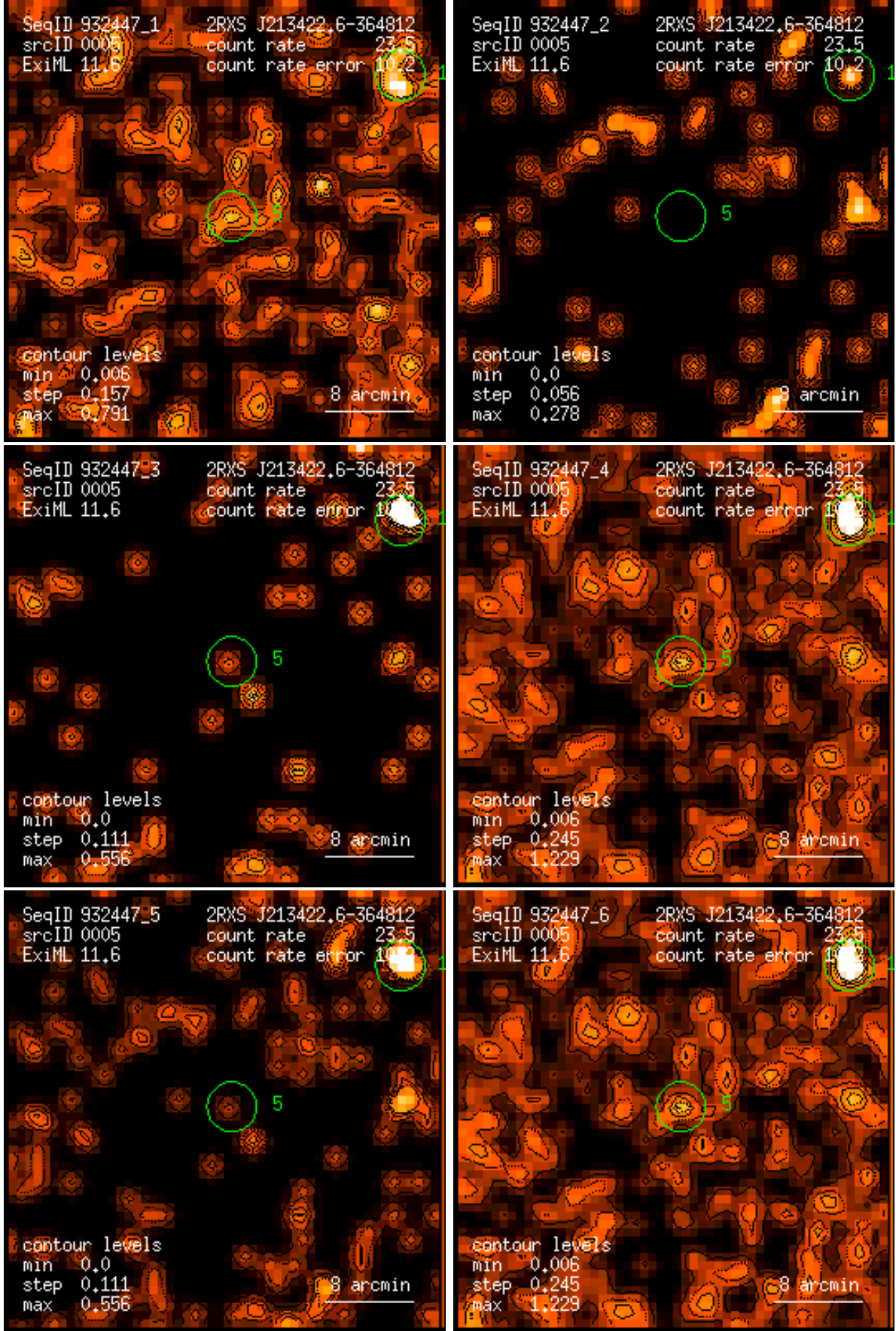
Figure 5: RASS 932447: detection 0005: band rate images, Gaussian filter: (1) PSPC channels 11 – 41, (2) 52 – 90, (3) 91 – 201, (4) 11 – 235, (5) 52 – 201, (6) 11 – 201. Broad band rates in counts/ks. Band rate contour levels in counts/ks/arcmin 2 .
