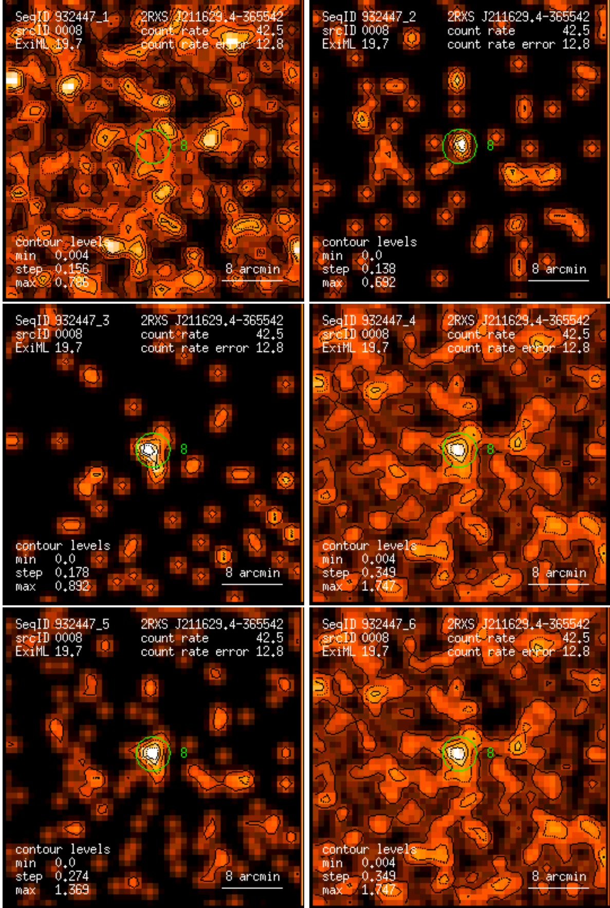
Figure 8: RASS 932447: detection 0008: band rate images, Gaussian filter: (1) PSPC channels 11 – 41, (2) 52 – 90, (3) 91 – 201, (4) 11 – 235, (5) 52 – 201, (6) 11 – 201. Broad band rates in counts/ks. Band rate contour levels in counts/ks/arcmin 2 .
