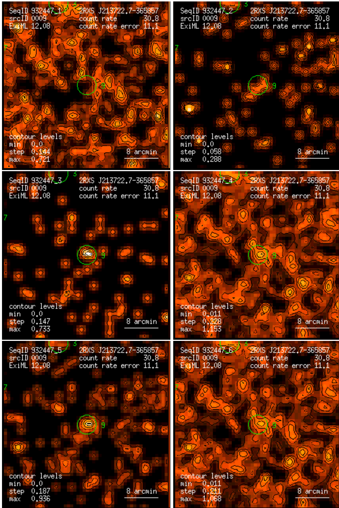
Figure 9: RASS 932447: detection 0009: band rate images, Gaussian filter: (1) PSPC channels 11 – 41, (2) 52 – 90, (3) 91 – 201, (4) 11 – 235, (5) 52 – 201, (6) 11 – 201. Broad band rates in counts/ks. Band rate contour levels in counts/ks/arcmin 2 .
