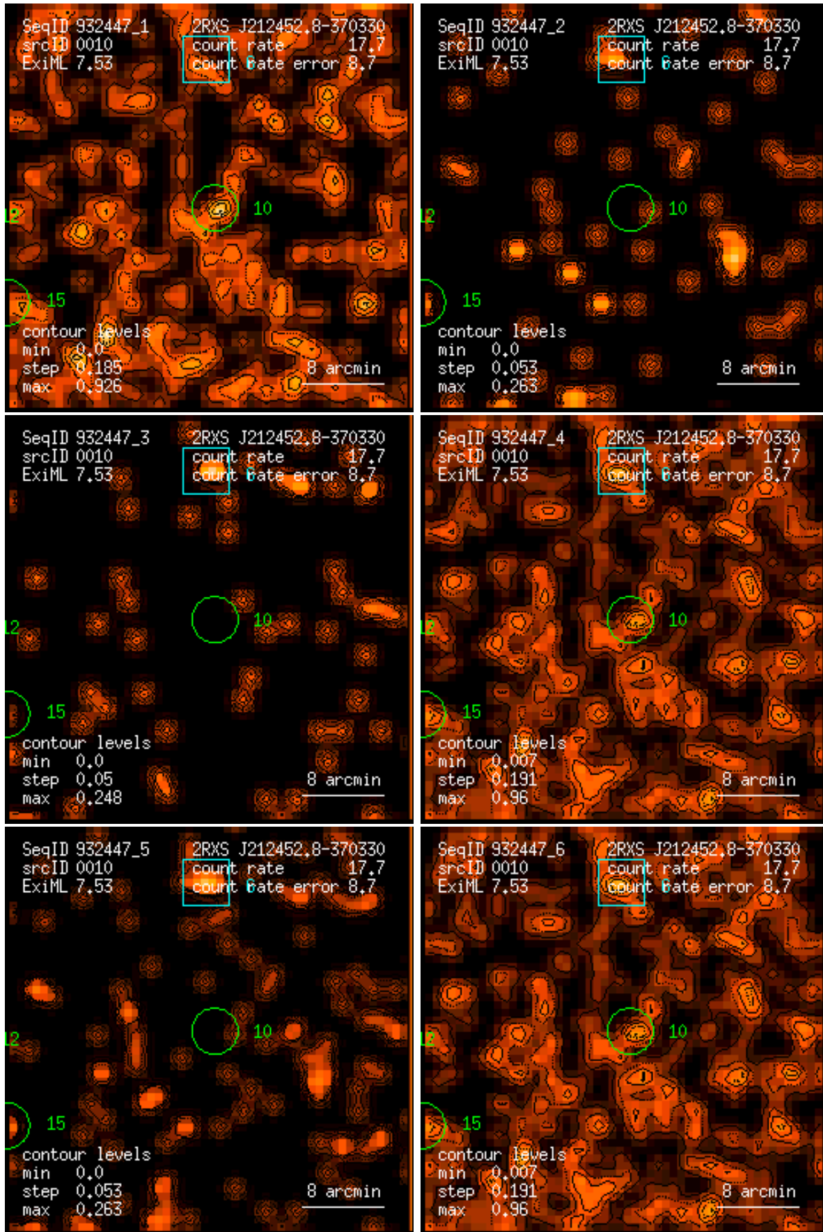
Figure 10: RASS 932447: detection 0010: band rate images, Gaussian filter: (1) PSPC channels 11 – 41, (2) 52 – 90, (3) 91 – 201, (4) 11 – 235, (5) 52 – 201, (6) 11 – 201. Broad band rates in counts/ks. Band rate contour levels in counts/ks/arcmin 2 .
