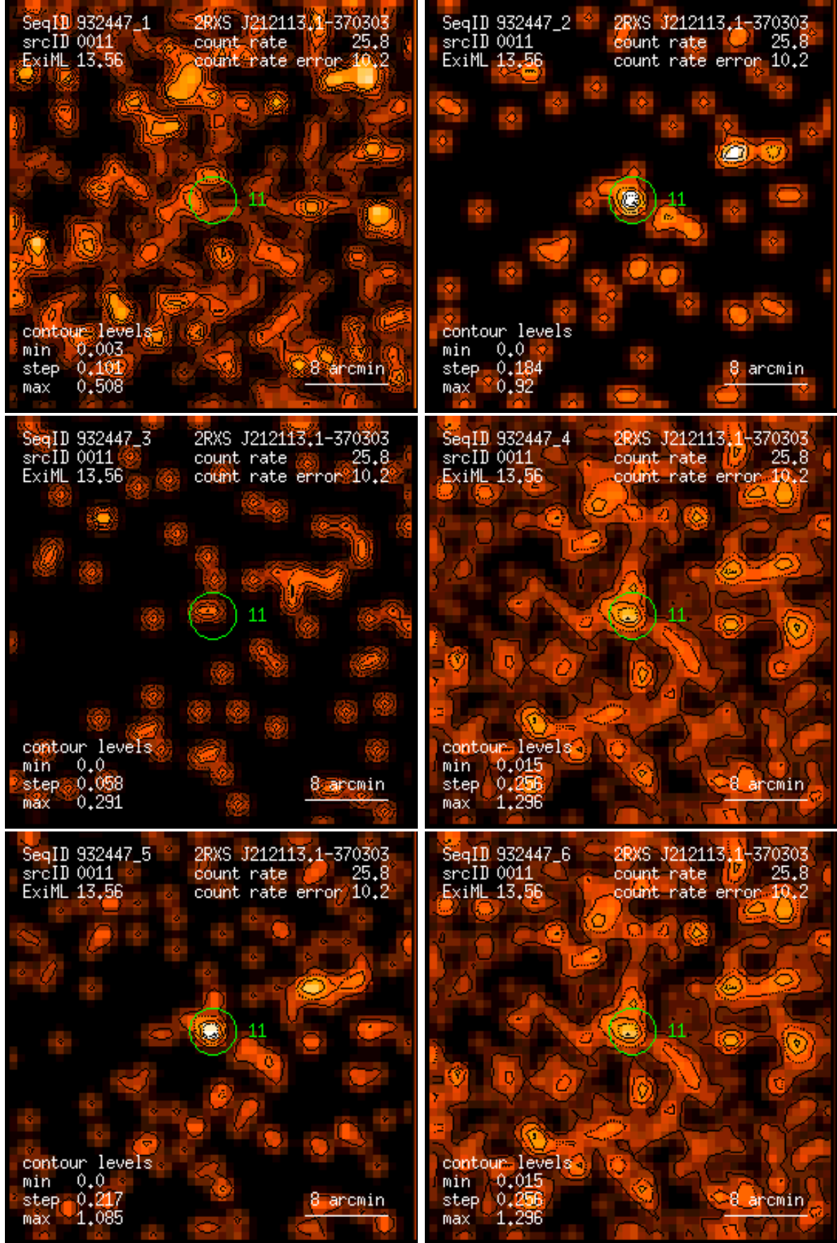
Figure 11: RASS 932447: detection 0011: band rate images, Gaussian filter: (1) PSPC channels 11 – 41, (2) 52 – 90, (3) 91 – 201, (4) 11 – 235, (5) 52 – 201, (6) 11 – 201. Broad band rates in counts/ks. Band rate contour levels in counts/ks/arcmin 2 .
