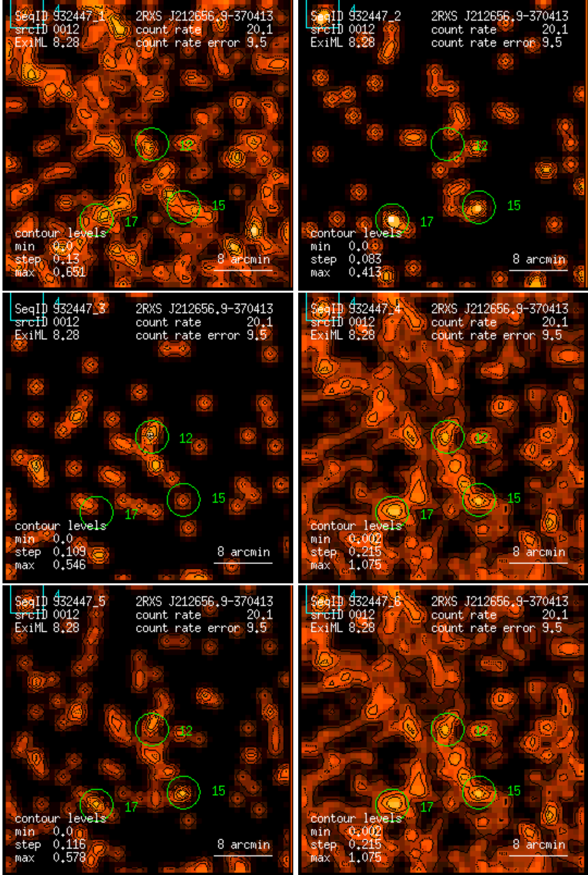
Figure 12: RASS 932447: detection 0012: band rate images, Gaussian filter: (1) PSPC channels 11 – 41, (2) 52 – 90, (3) 91 – 201, (4) 11 – 235, (5) 52 – 201, (6) 11 – 201. Broad band rates in counts/ks. Band rate contour levels in counts/ks/arcmin 2 .
