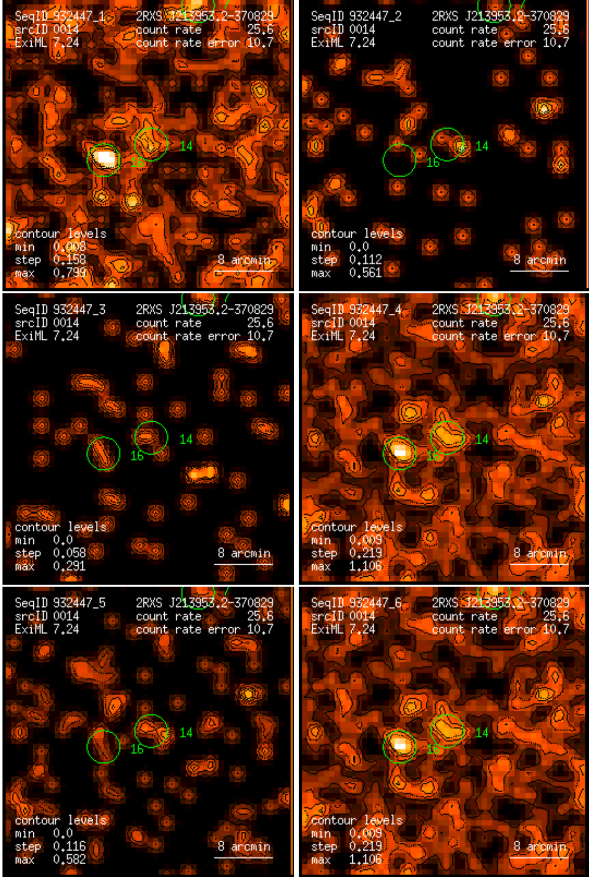
Figure 14: RASS 932447: detection 0014: band rate images, Gaussian filter: (1) PSPC channels 11 – 41, (2) 52 – 90, (3) 91 – 201, (4) 11 – 235, (5) 52 – 201, (6) 11 – 201. Broad band rates in counts/ks. Band rate contour levels in counts/ks/arcmin 2 .
