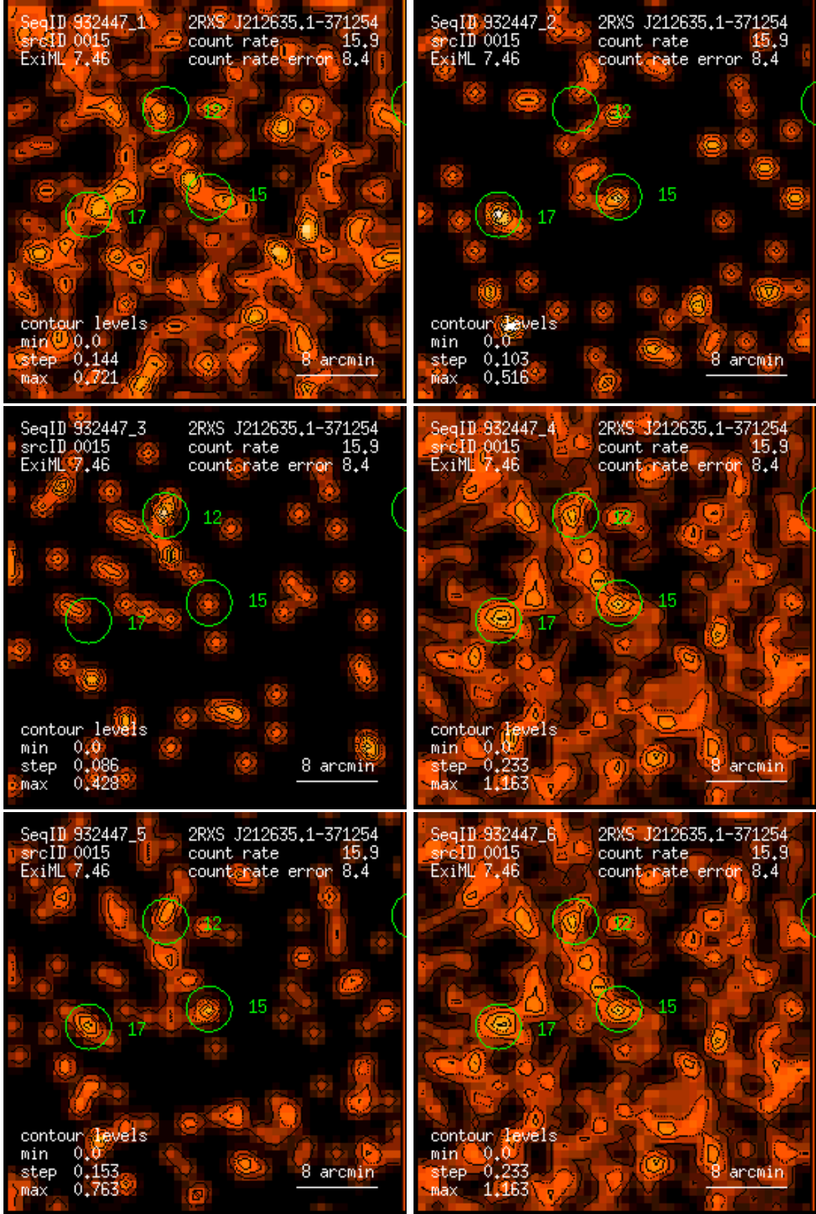
Figure 15: RASS 932447: detection 0015: band rate images, Gaussian filter: (1) PSPC channels 11 – 41, (2) 52 – 90, (3) 91 – 201, (4) 11 – 235, (5) 52 – 201, (6) 11 – 201. Broad band rates in counts/ks. Band rate contour levels in counts/ks/arcmin 2 .
