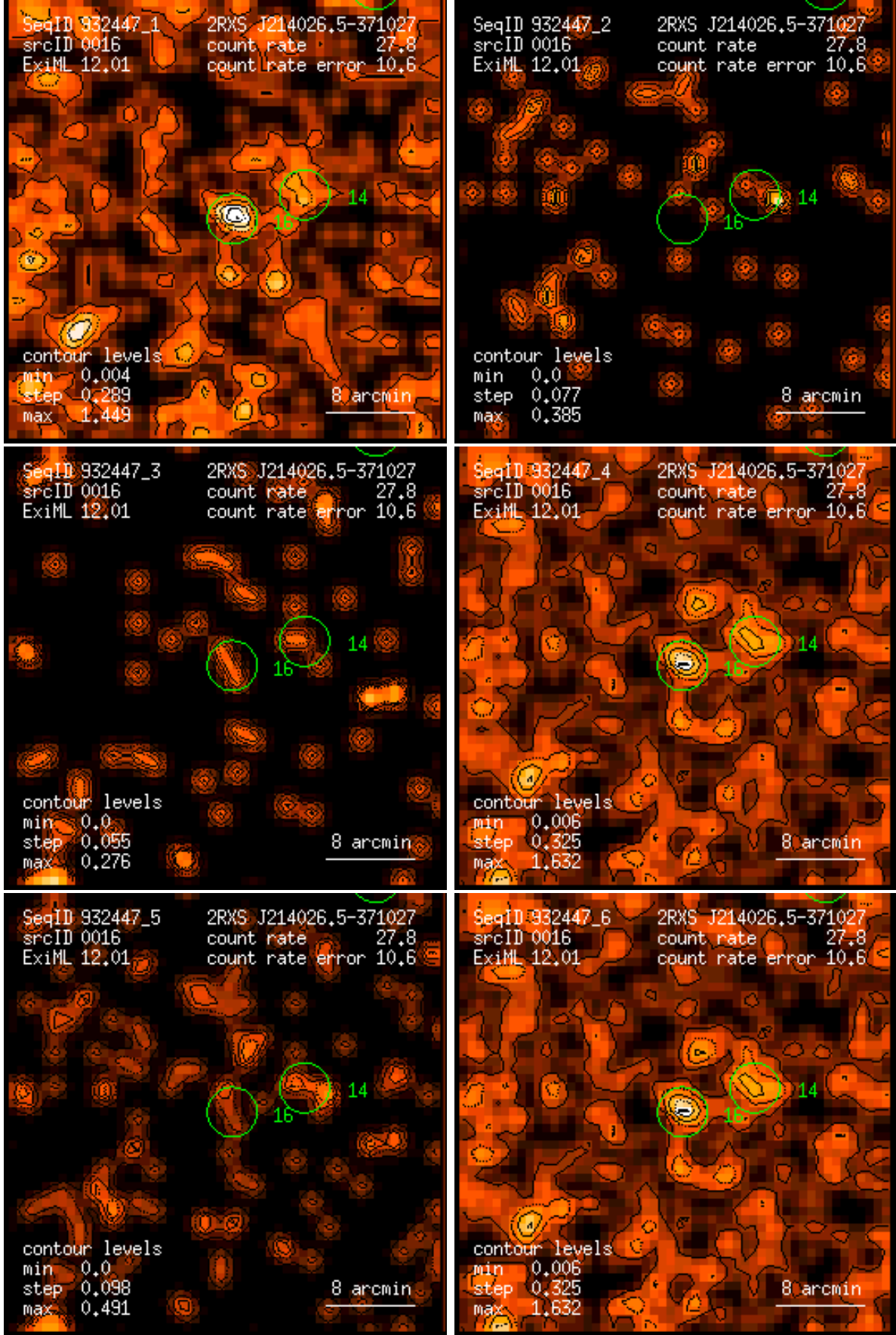
Figure 16: RASS 932447: detection 0016: band rate images, Gaussian filter: (1) PSPC channels 11 – 41, (2) 52 – 90, (3) 91 – 201, (4) 11 – 235, (5) 52 – 201, (6) 11 – 201. Broad band rates in counts/ks. Band rate contour levels in counts/ks/arcmin 2 .
