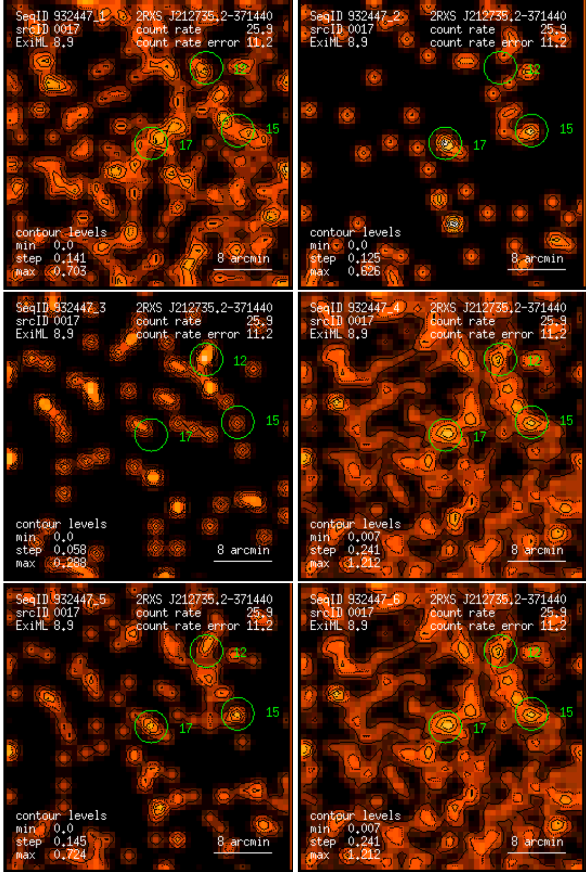
Figure 17: RASS 932447: detection 0017: band rate images, Gaussian filter: (1) PSPC channels 11 – 41, (2) 52 – 90, (3) 91 – 201, (4) 11 – 235, (5) 52 – 201, (6) 11 – 201. Broad band rates in counts/ks. Band rate contour levels in counts/ks/arcmin 2 .
