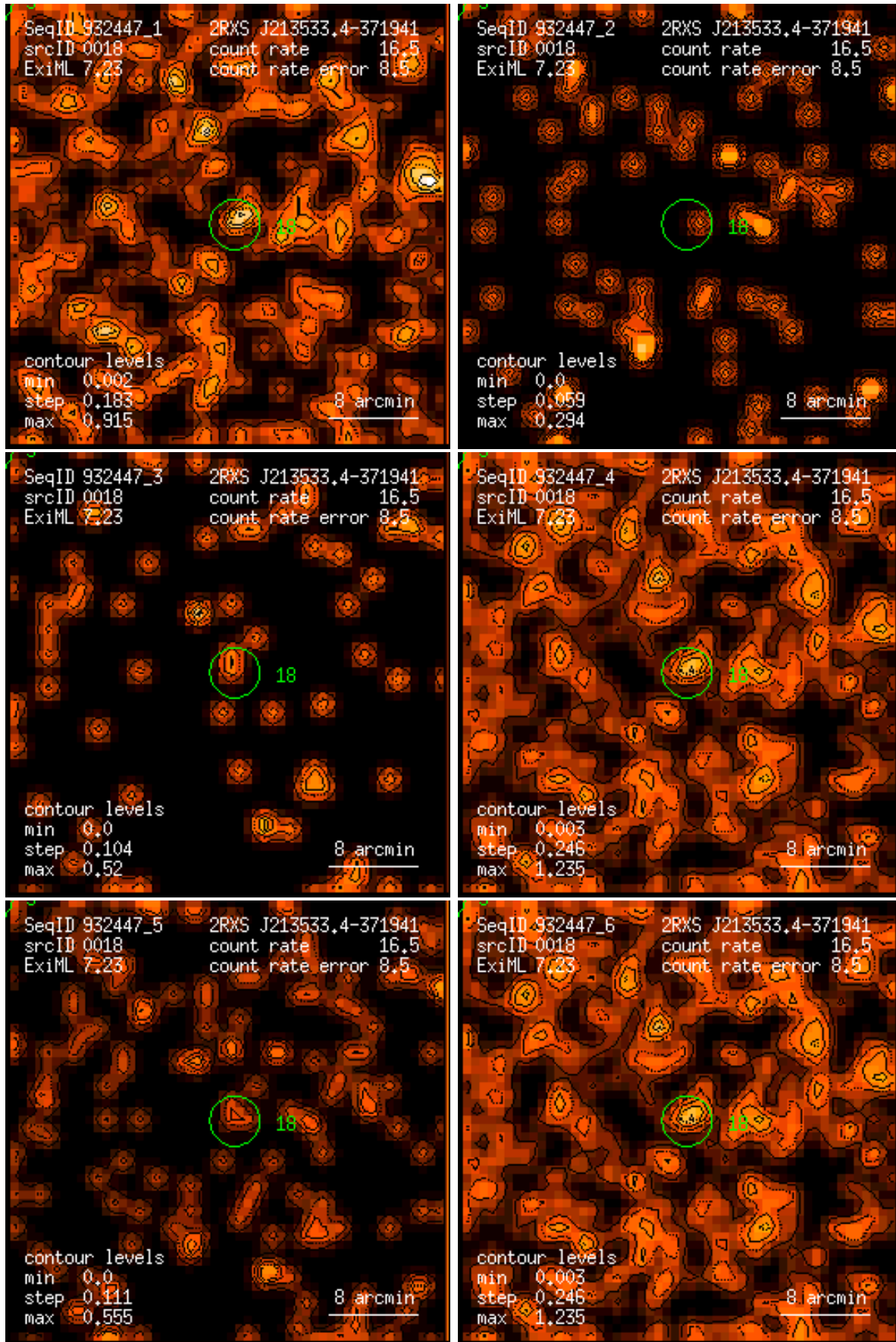
Figure 18: RASS 932447: detection 0018: band rate images, Gaussian filter: (1) PSPC channels 11 – 41, (2) 52 – 90, (3) 91 – 201, (4) 11 – 235, (5) 52 – 201, (6) 11 – 201. Broad band rates in counts/ks. Band rate contour levels in counts/ks/arcmin 2 .
