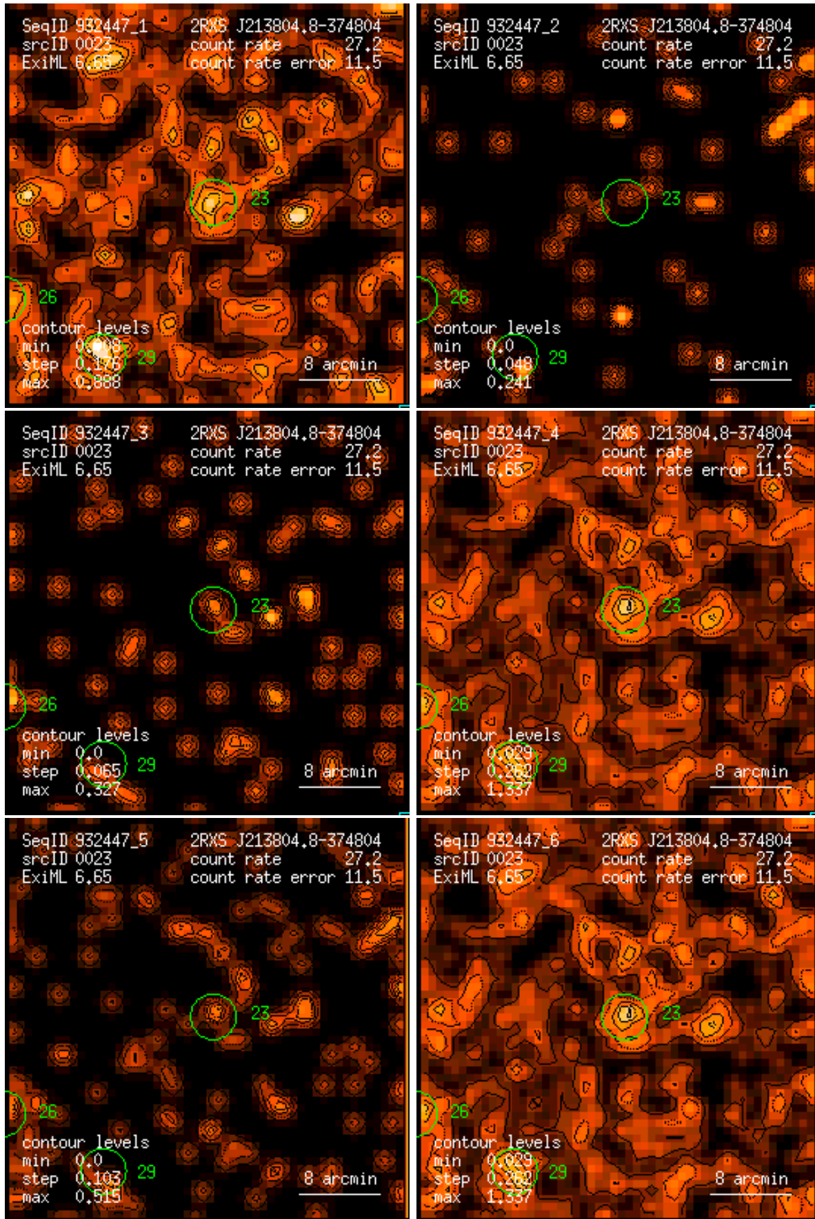
Figure 23: RASS 932447: detection 0023: band rate images, Gaussian filter: (1) PSPC channels 11 – 41, (2) 52 – 90, (3) 91 – 201, (4) 11 – 235, (5) 52 – 201, (6) 11 – 201. Broad band rates in counts/ks. Band rate contour levels in counts/ks/arcmin 2 .
