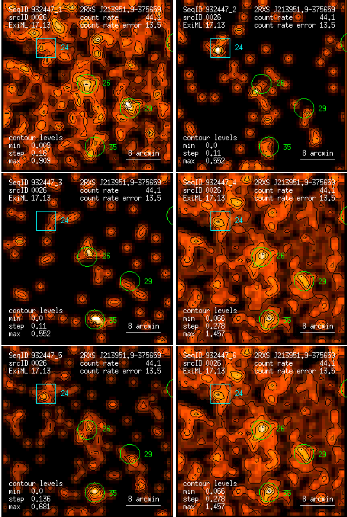
Figure 26: RASS 932447: detection 0026: band rate images, Gaussian filter: (1) PSPC channels 11 – 41, (2) 52 – 90, (3) 91 – 201, (4) 11 – 235, (5) 52 – 201, (6) 11 – 201. Broad band rates in counts/ks. Band rate contour levels in counts/ks/arcmin 2 .
