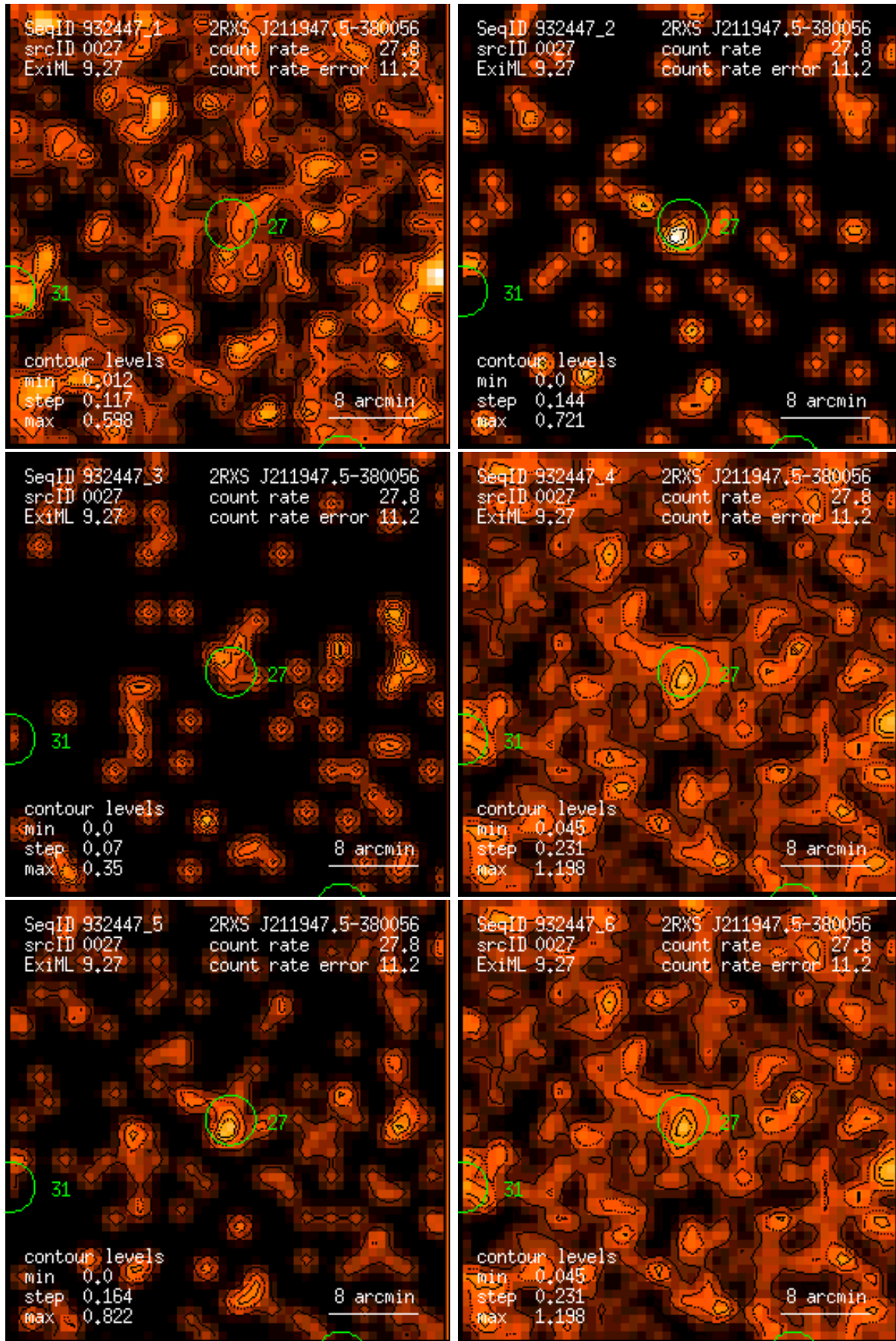
Figure 27: RASS 932447: detection 0027: band rate images, Gaussian filter: (1) PSPC channels 11 – 41, (2) 52 – 90, (3) 91 – 201, (4) 11 – 235, (5) 52 – 201, (6) 11 – 201. Broad band rates in counts/ks. Band rate contour levels in counts/ks/arcmin 2 .
