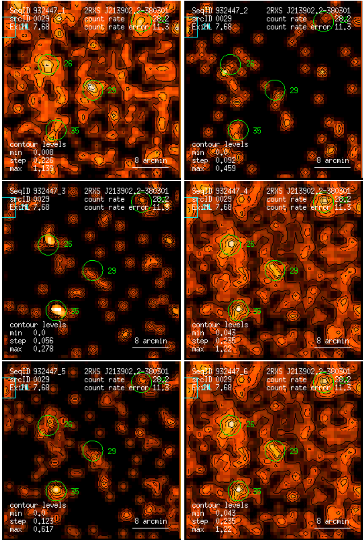
Figure 29: RASS 932447: detection 0029: band rate images, Gaussian filter: (1) PSPC channels 11 – 41, (2) 52 – 90, (3) 91 – 201, (4) 11 – 235, (5) 52 – 201, (6) 11 – 201. Broad band rates in counts/ks. Band rate contour levels in counts/ks/arcmin 2 .
