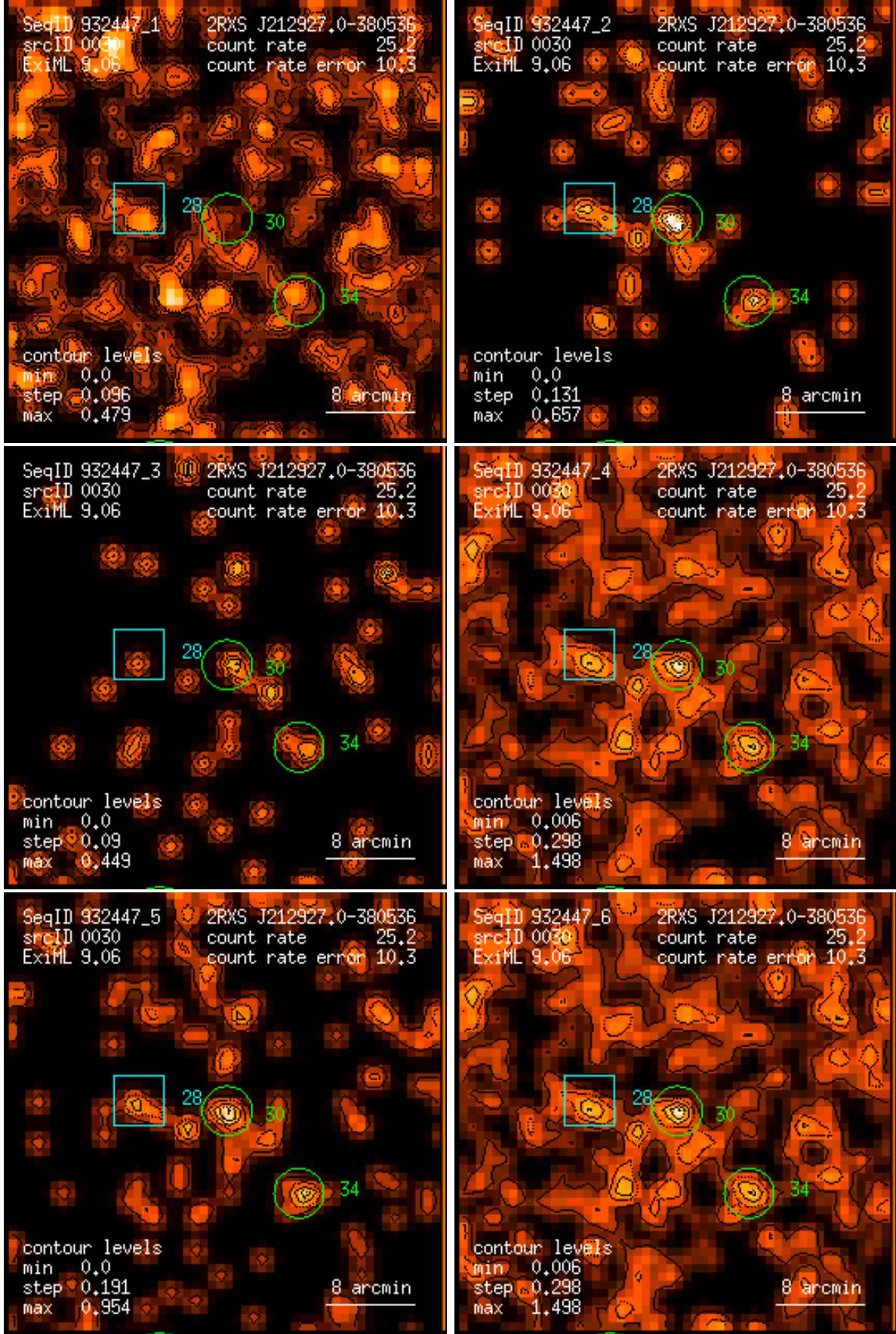
Figure 30: RASS 932447: detection 0030: band rate images, Gaussian filter: (1) PSPC channels 11 – 41, (2) 52 – 90, (3) 91 – 201, (4) 11 – 235, (5) 52 – 201, (6) 11 – 201. Broad band rates in counts/ks. Band rate contour levels in counts/ks/arcmin 2 .
