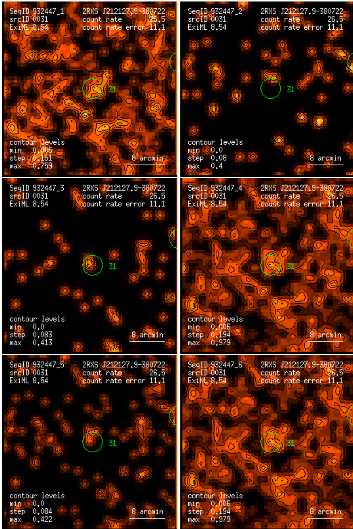
Figure 31: RASS 932447: detection 0031: band rate images, Gaussian filter: (1) PSPC channels 11 – 41, (2) 52 – 90, (3) 91 – 201, (4) 11 – 235, (5) 52 – 201, (6) 11 – 201. Broad band rates in counts/ks. Band rate contour levels in counts/ks/arcmin 2 .
