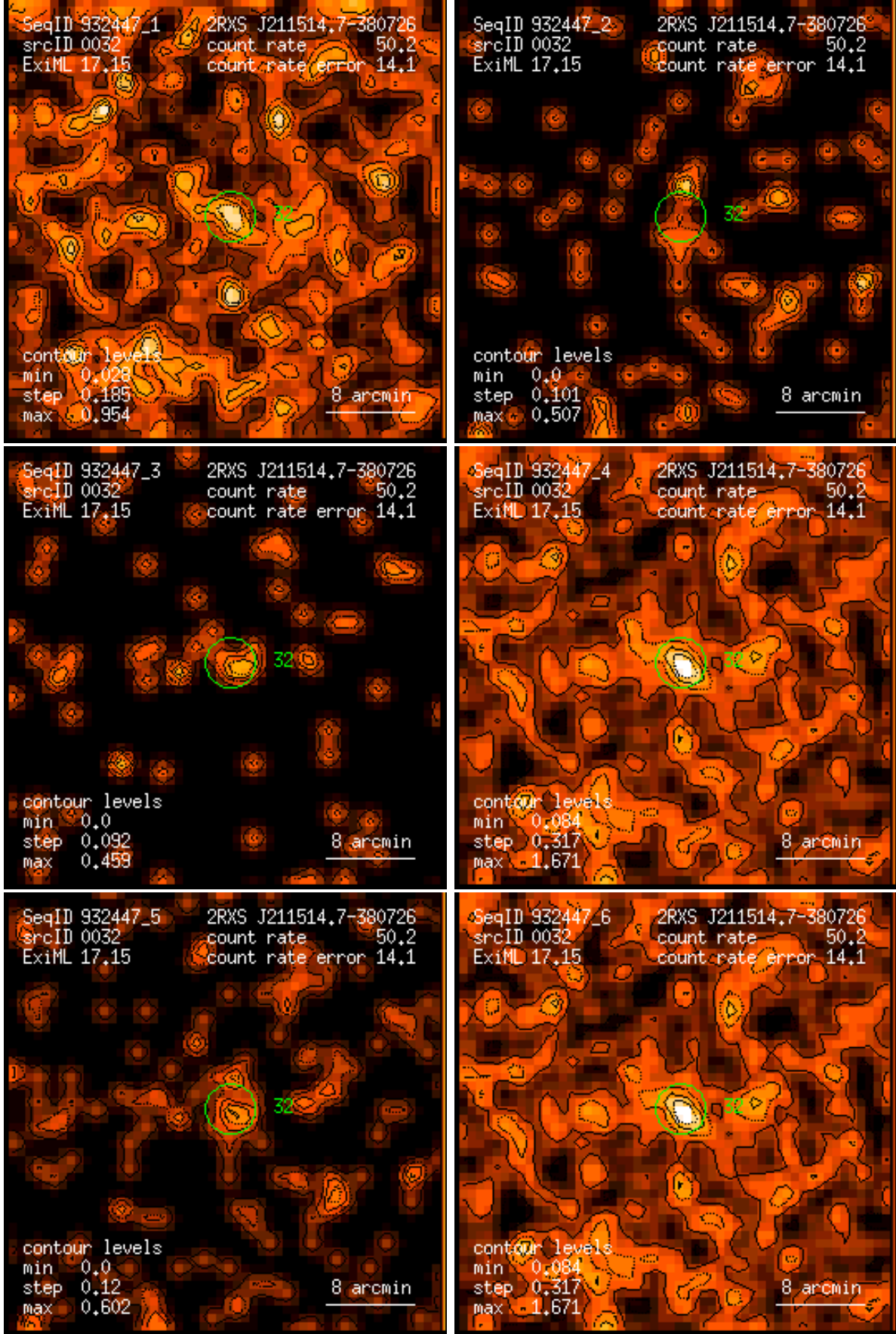
Figure 32: RASS 932447: detection 0032: band rate images, Gaussian filter: (1) PSPC channels 11 – 41, (2) 52 – 90, (3) 91 – 201, (4) 11 – 235, (5) 52 – 201, (6) 11 – 201. Broad band rates in counts/ks. Band rate contour levels in counts/ks/arcmin 2 .
