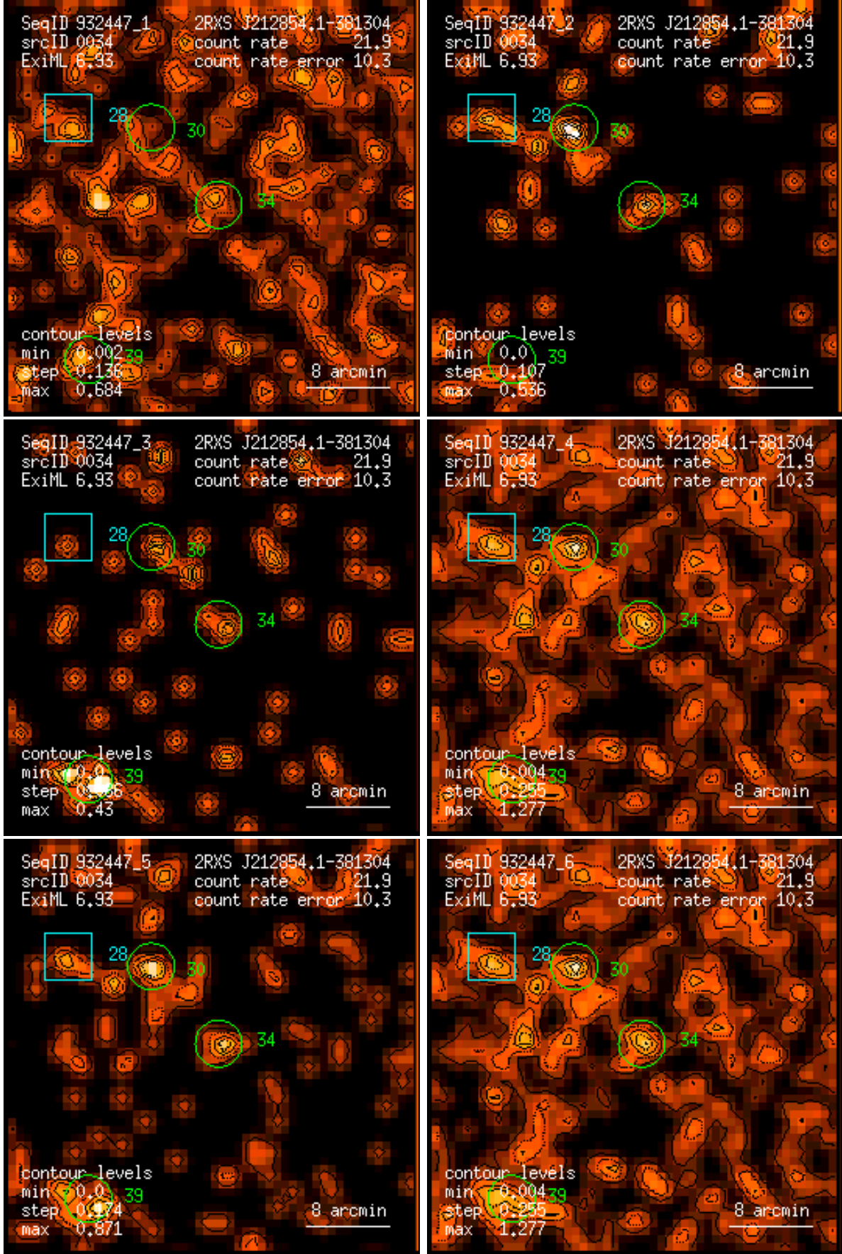
Figure 34: RASS 932447: detection 0034: band rate images, Gaussian filter: (1) PSPC channels 11 – 41, (2) 52 – 90, (3) 91 – 201, (4) 11 – 235, (5) 52 – 201, (6) 11 – 201. Broad band rates in counts/ks. Band rate contour levels in counts/ks/arcmin 2 .
