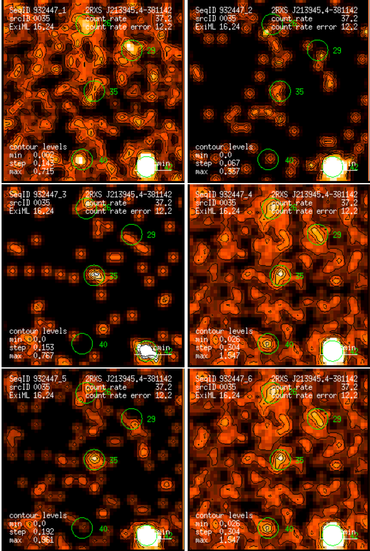
Figure 35: RASS 932447: detection 0035: band rate images, Gaussian filter: (1) PSPC channels 11 – 41, (2) 52 – 90, (3) 91 – 201, (4) 11 – 235, (5) 52 – 201, (6) 11 – 201. Broad band rates in counts/ks. Band rate contour levels in counts/ks/arcmin 2 .
