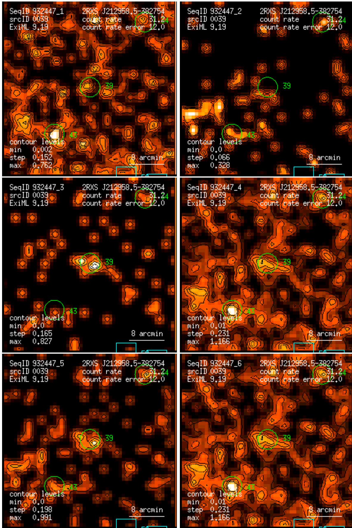
Figure 39: RASS 932447: detection 0039: band rate images, Gaussian filter: (1) PSPC channels 11 – 41, (2) 52 – 90, (3) 91 – 201, (4) 11 – 235, (5) 52 – 201, (6) 11 – 201. Broad band rates in counts/ks. Band rate contour levels in counts/ks/arcmin 2 .
