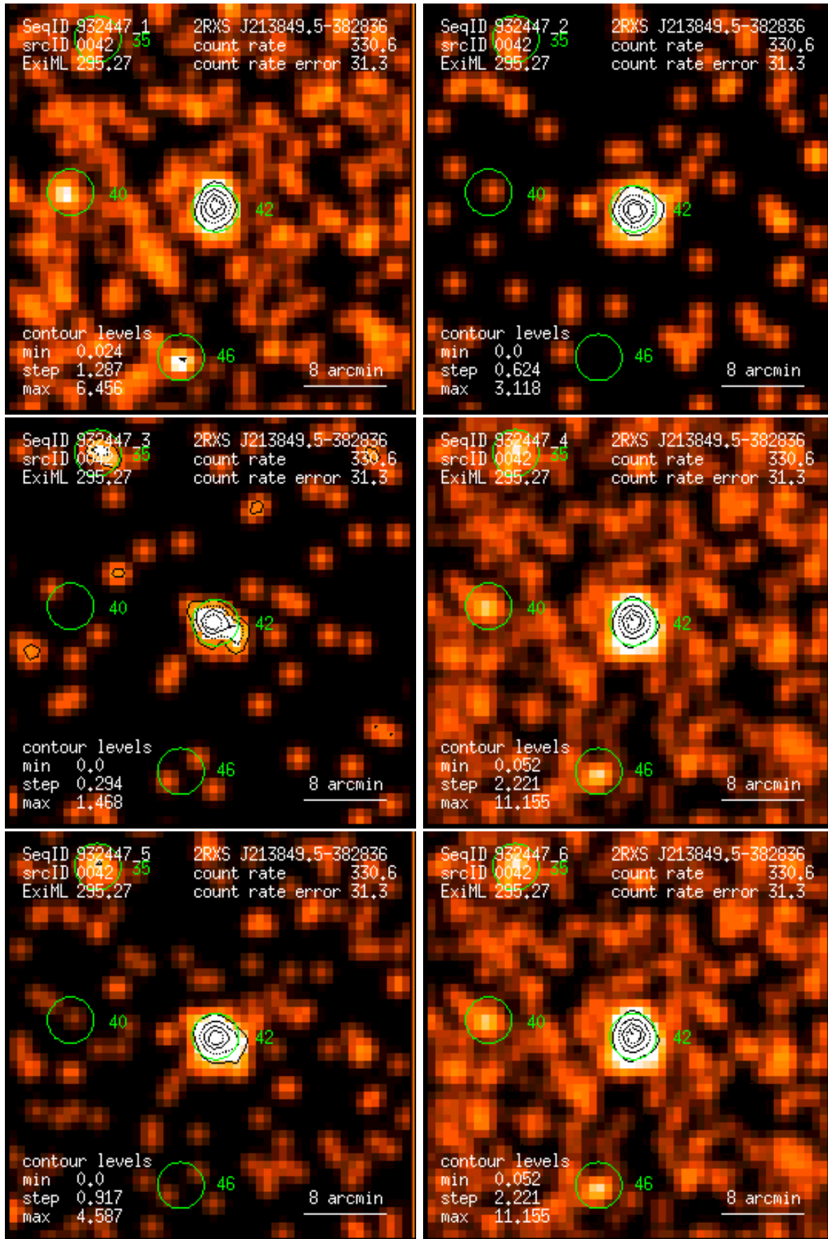
Figure 42: RASS 932447: detection 0042: band rate images, Gaussian filter: (1) PSPC channels 11 – 41, (2) 52 – 90, (3) 91 – 201, (4) 11 – 235, (5) 52 – 201, (6) 11 – 201. Broad band rates in counts/ks. Band rate contour levels in counts/ks/arcmin 2 .
