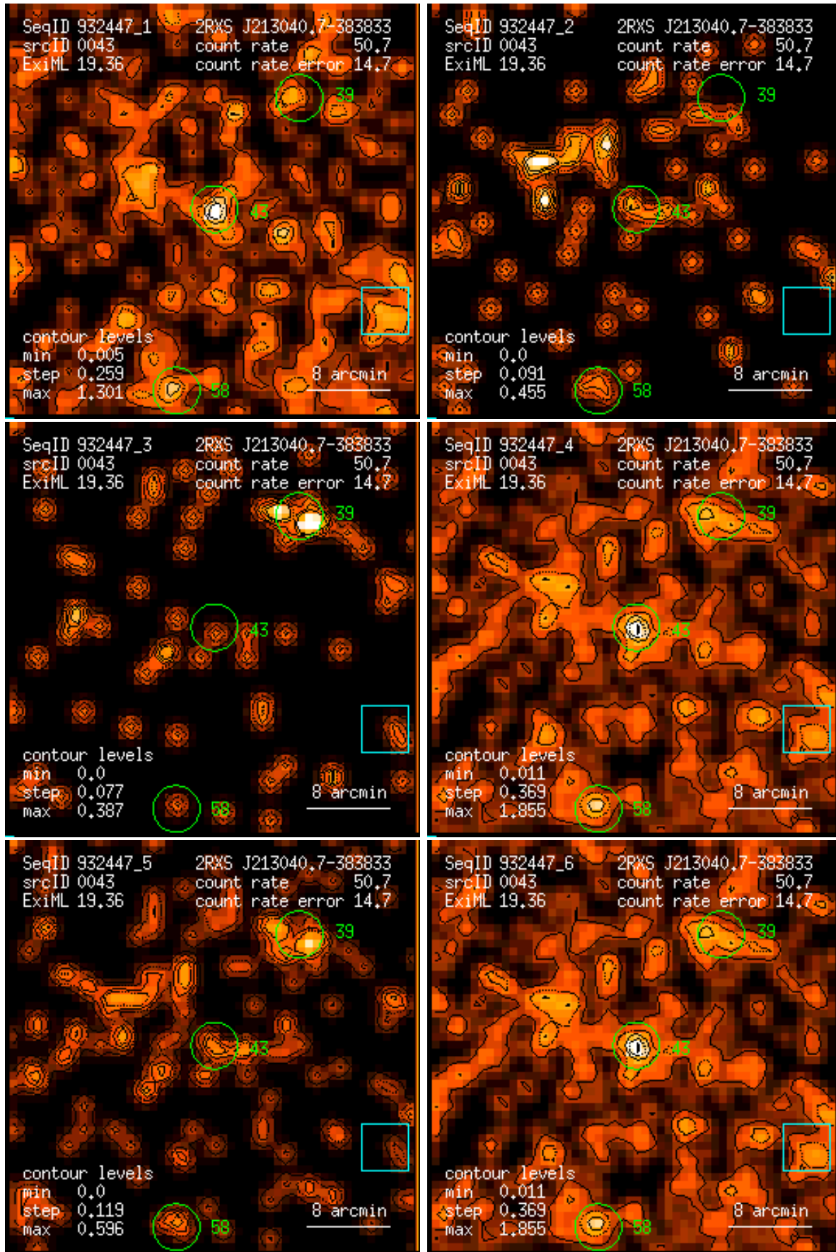
Figure 43: RASS 932447: detection 0043: band rate images, Gaussian filter: (1) PSPC channels 11 – 41, (2) 52 – 90, (3) 91 – 201, (4) 11 – 235, (5) 52 – 201, (6) 11 – 201. Broad band rates in counts/ks. Band rate contour levels in counts/ks/arcmin 2 .
