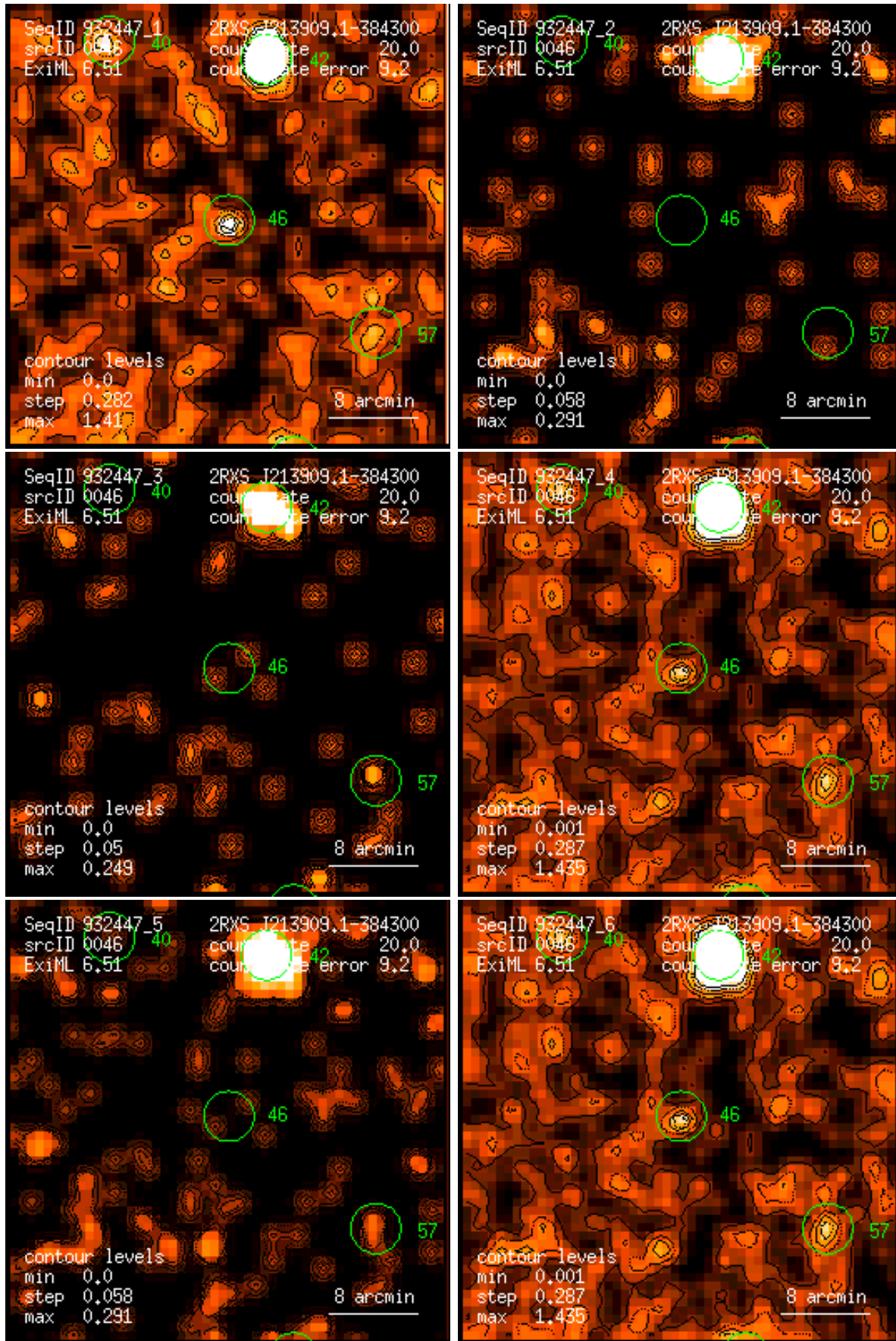
Figure 46: RASS 932447: detection 0046: band rate images, Gaussian filter: (1) PSPC channels 11 – 41, (2) 52 – 90, (3) 91 – 201, (4) 11 – 235, (5) 52 – 201, (6) 11 – 201. Broad band rates in counts/ks. Band rate contour levels in counts/ks/arcmin 2 .
