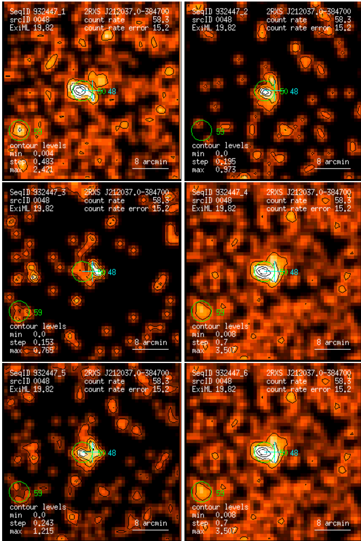
Figure 48: RASS 932447: detection 0048: band rate images, Gaussian filter: (1) PSPC channels 11 – 41, (2) 52 – 90, (3) 91 – 201, (4) 11 – 235, (5) 52 – 201, (6) 11 – 201. Broad band rates in counts/ks. Band rate contour levels in counts/ks/arcmin 2 .
