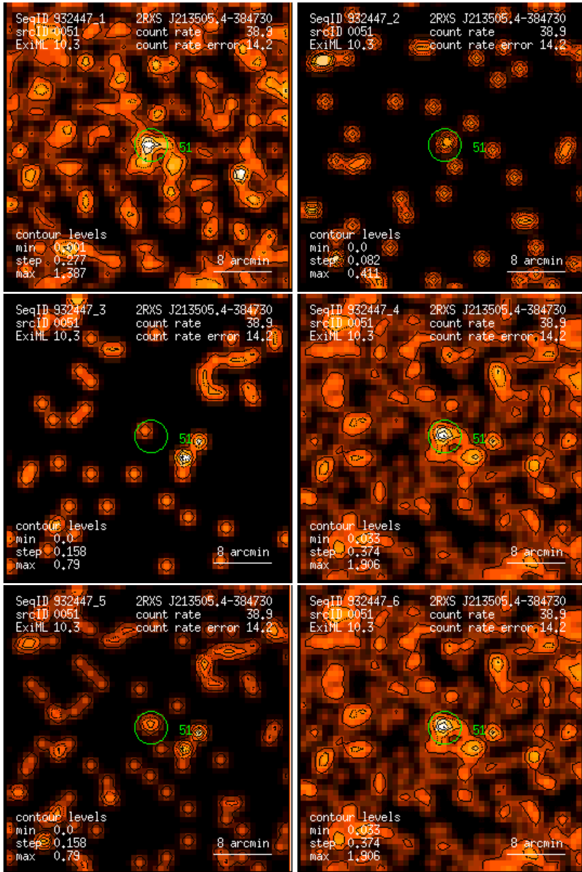
Figure 51: RASS 932447: detection 0051: band rate images, Gaussian filter: (1) PSPC channels 11 – 41, (2) 52 – 90, (3) 91 – 201, (4) 11 – 235, (5) 52 – 201, (6) 11 – 201. Broad band rates in counts/ks. Band rate contour levels in counts/ks/arcmin 2 .
