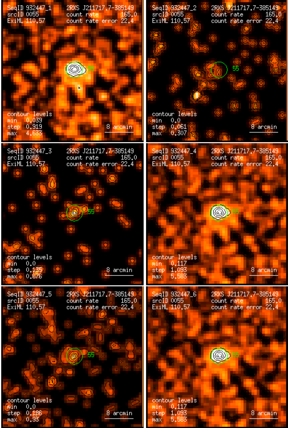
Figure 55: RASS 932447: detection 0055: band rate images, Gaussian filter: (1) PSPC channels 11 – 41, (2) 52 – 90, (3) 91 – 201, (4) 11 – 235, (5) 52 – 201, (6) 11 – 201. Broad band rates in counts/ks. Band rate contour levels in counts/ks/arcmin 2 .
