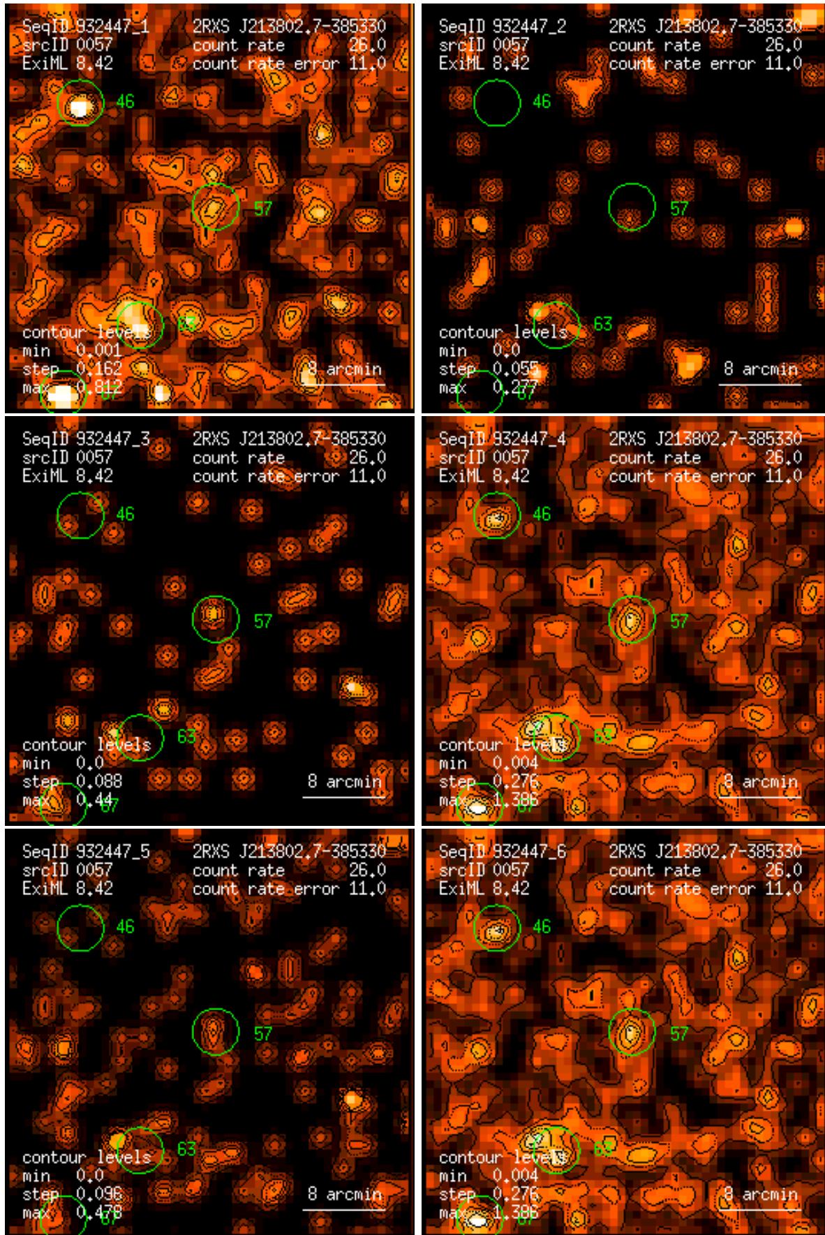
Figure 57: RASS 932447: detection 0057: band rate images, Gaussian filter: (1) PSPC channels 11 – 41, (2) 52 – 90, (3) 91 – 201, (4) 11 – 235, (5) 52 – 201, (6) 11 – 201. Broad band rates in counts/ks. Band rate contour levels in counts/ks/arcmin 2 .
