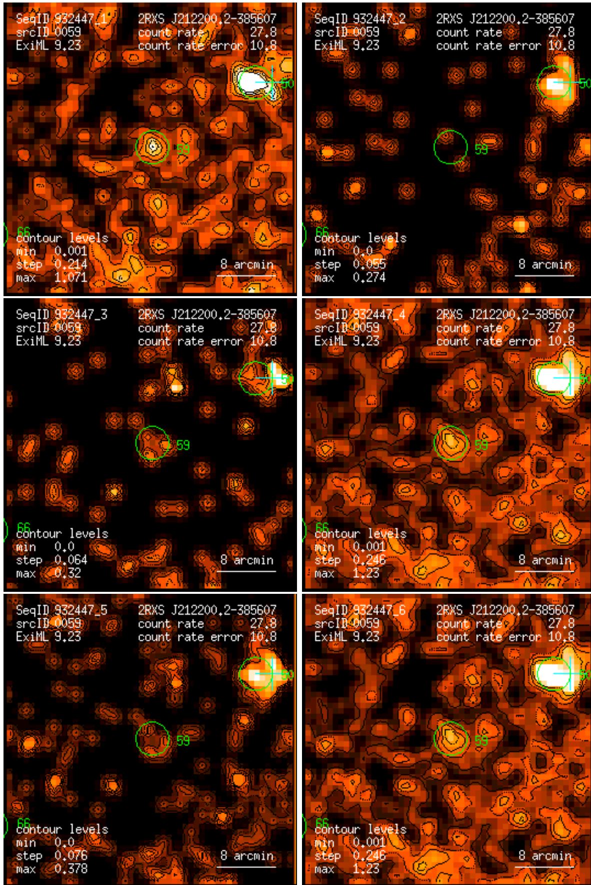
Figure 59: RASS 932447: detection 0059: band rate images, Gaussian filter: (1) PSPC channels 11 – 41, (2) 52 – 90, (3) 91 – 201, (4) 11 – 235, (5) 52 – 201, (6) 11 – 201. Broad band rates in counts/ks. Band rate contour levels in counts/ks/arcmin 2 .
