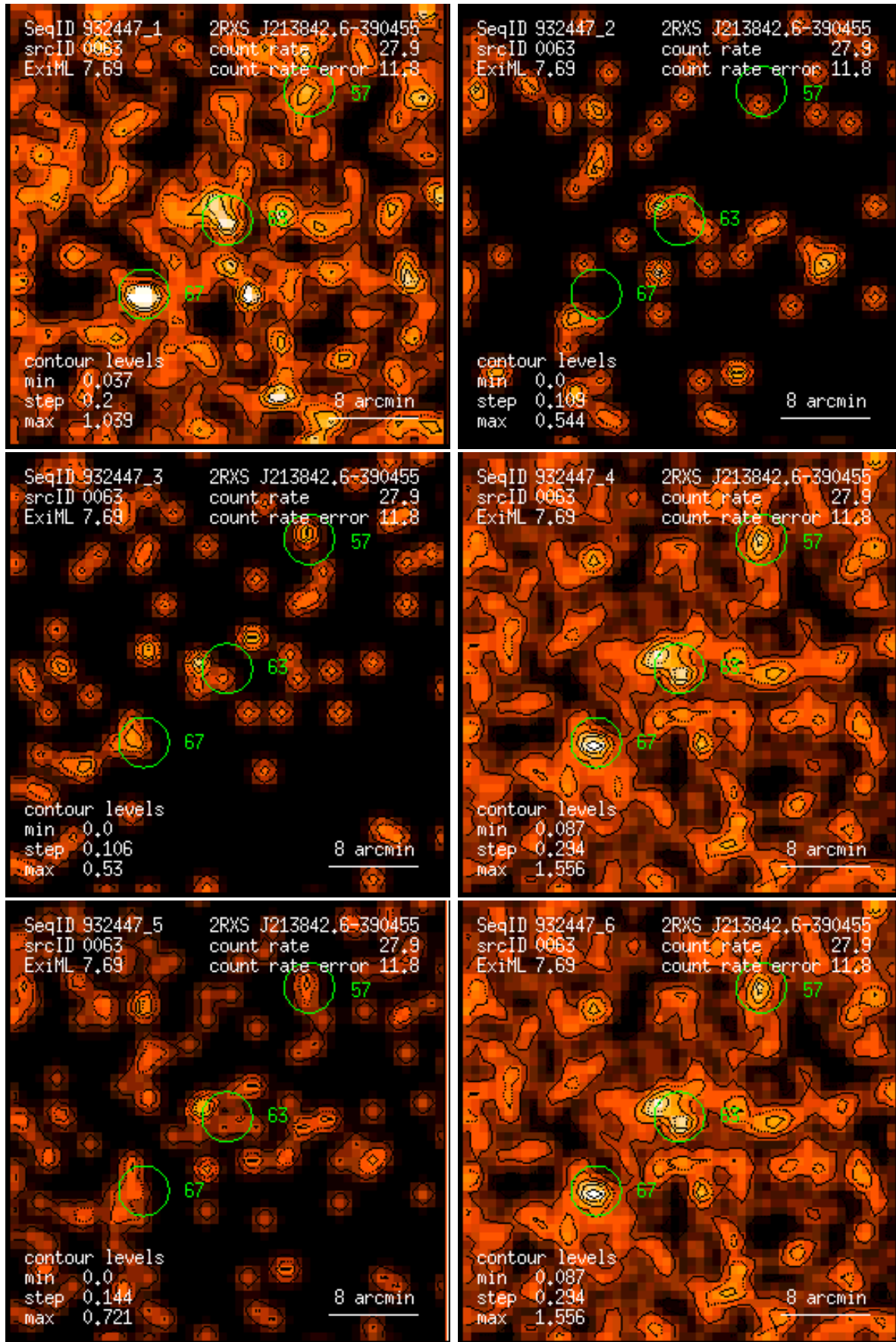
Figure 63: RASS 932447: detection 0063: band rate images, Gaussian filter: (1) PSPC channels 11 – 41, (2) 52 – 90, (3) 91 – 201, (4) 11 – 235, (5) 52 – 201, (6) 11 – 201. Broad band rates in counts/ks. Band rate contour levels in counts/ks/arcmin 2 .
