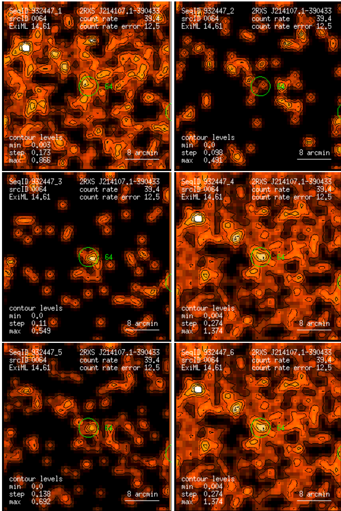
Figure 64: RASS 932447: detection 0064: band rate images, Gaussian filter: (1) PSPC channels 11 – 41, (2) 52 – 90, (3) 91 – 201, (4) 11 – 235, (5) 52 – 201, (6) 11 – 201. Broad band rates in counts/ks. Band rate contour levels in counts/ks/arcmin 2 .
