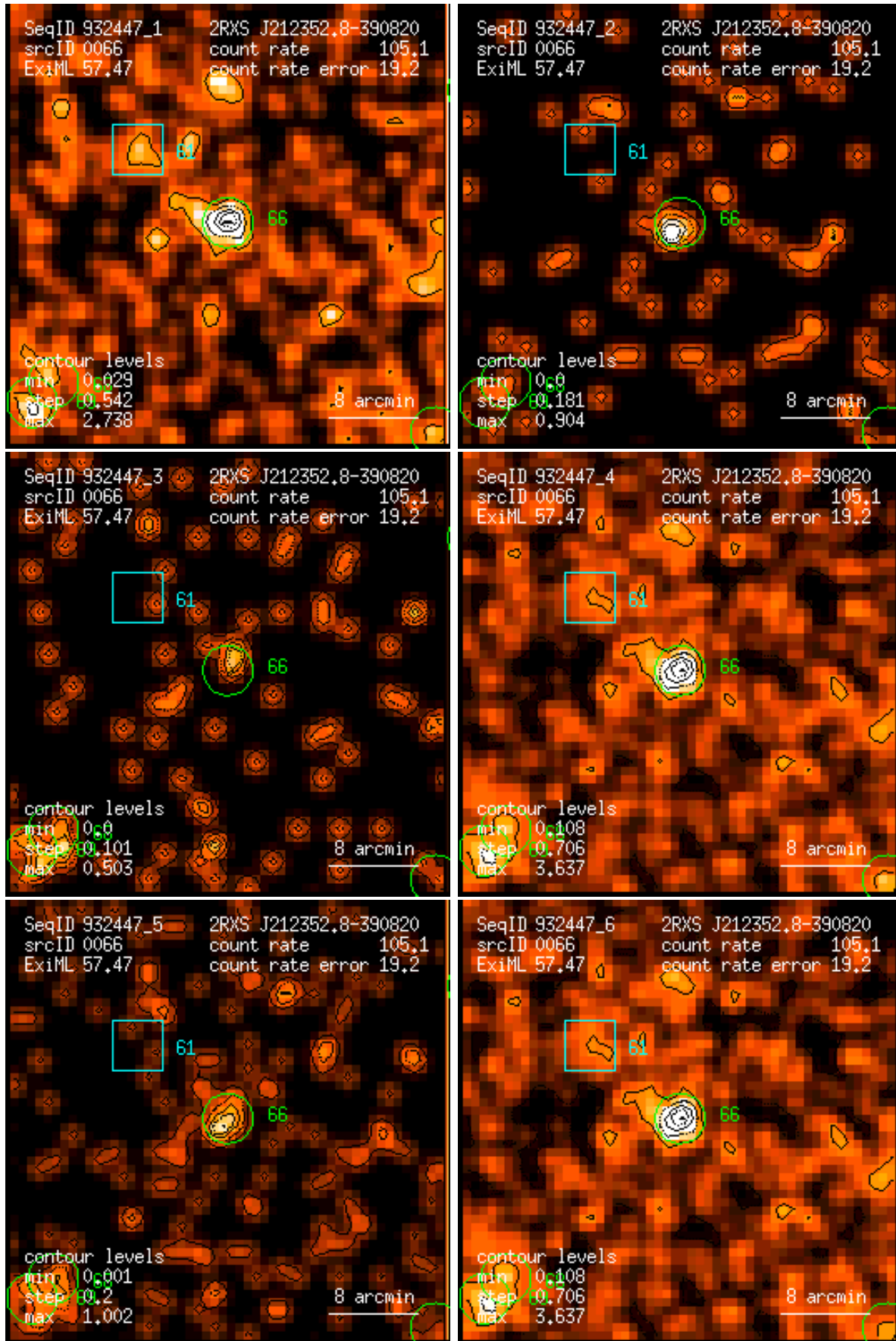
Figure 66: RASS 932447: detection 0066: band rate images, Gaussian filter: (1) PSPC channels 11 – 41, (2) 52 – 90, (3) 91 – 201, (4) 11 – 235, (5) 52 – 201, (6) 11 – 201. Broad band rates in counts/ks. Band rate contour levels in counts/ks/arcmin 2 .
