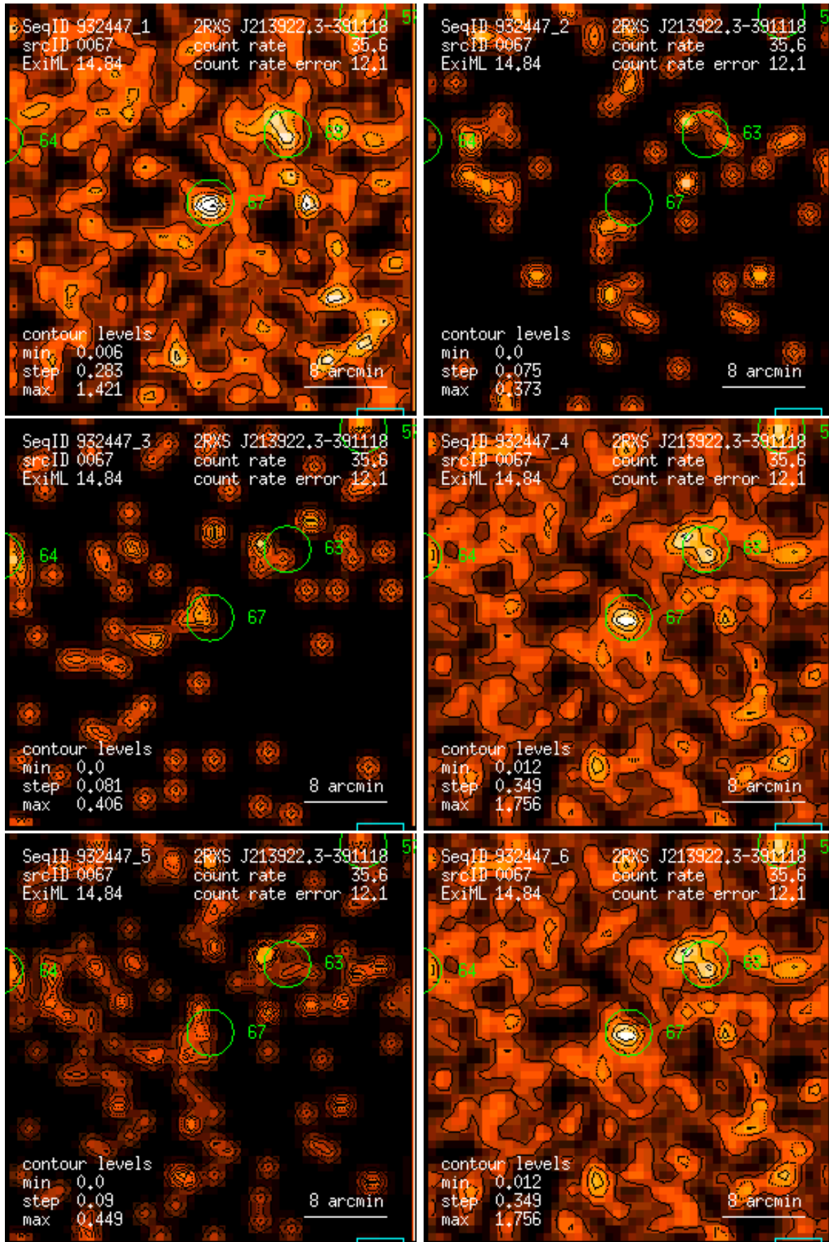
Figure 67: RASS 932447: detection 0067: band rate images, Gaussian filter: (1) PSPC channels 11 – 41, (2) 52 – 90, (3) 91 – 201, (4) 11 – 235, (5) 52 – 201, (6) 11 – 201. Broad band rates in counts/ks. Band rate contour levels in counts/ks/arcmin 2 .
