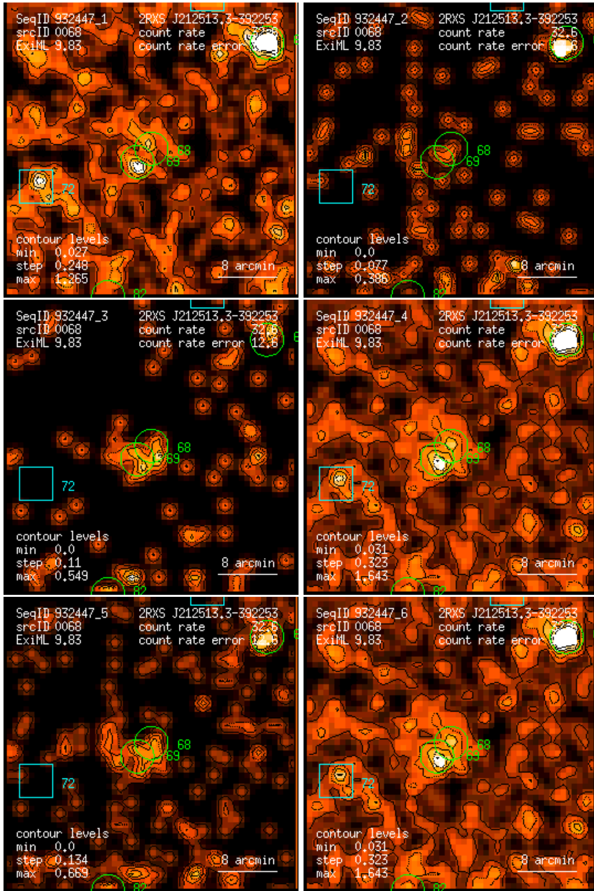
Figure 68: RASS 932447: detection 0068: band rate images, Gaussian filter: (1) PSPC channels 11 – 41, (2) 52 – 90, (3) 91 – 201, (4) 11 – 235, (5) 52 – 201, (6) 11 – 201. Broad band rates in counts/ks. Band rate contour levels in counts/ks/arcmin 2 .
