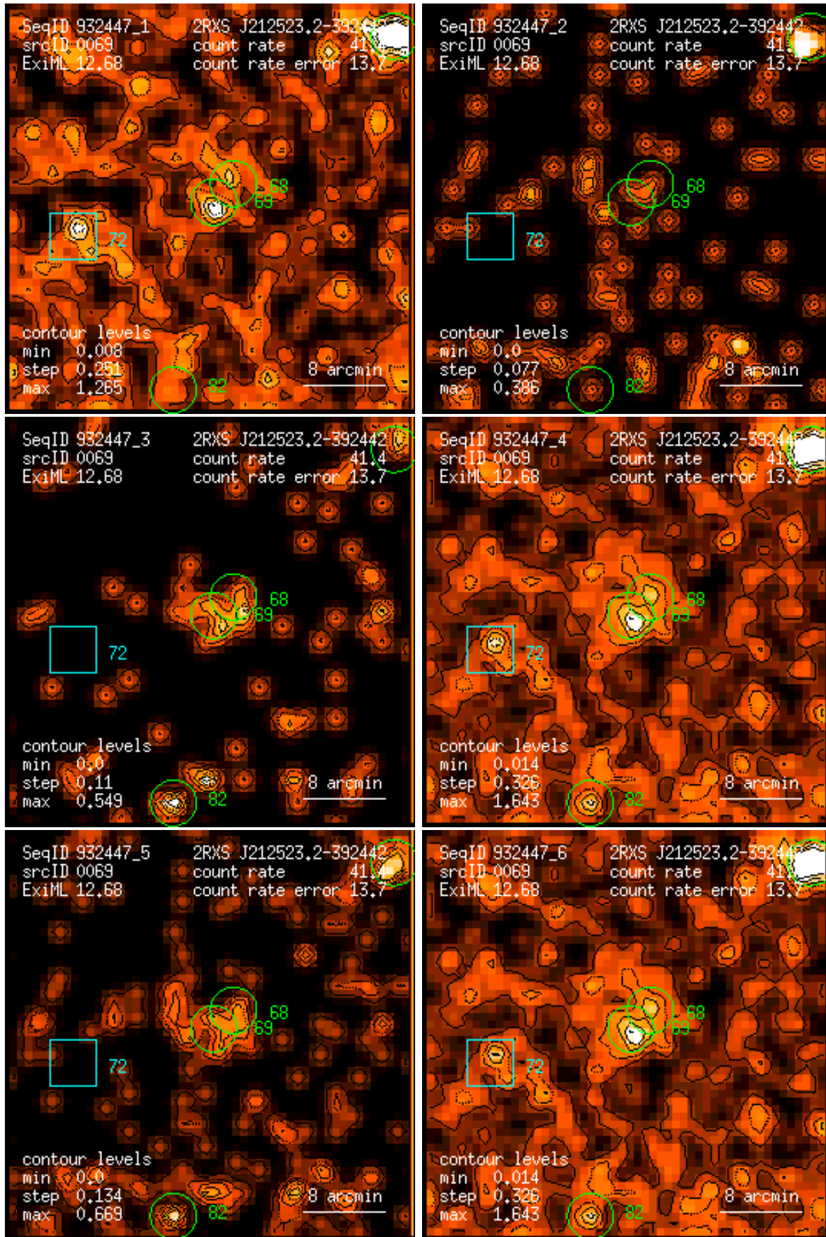
Figure 69: RASS 932447: detection 0069: band rate images, Gaussian filter: (1) PSPC channels 11 – 41, (2) 52 – 90, (3) 91 – 201, (4) 11 – 235, (5) 52 – 201, (6) 11 – 201. Broad band rates in counts/ks. Band rate contour levels in counts/ks/arcmin 2 .
