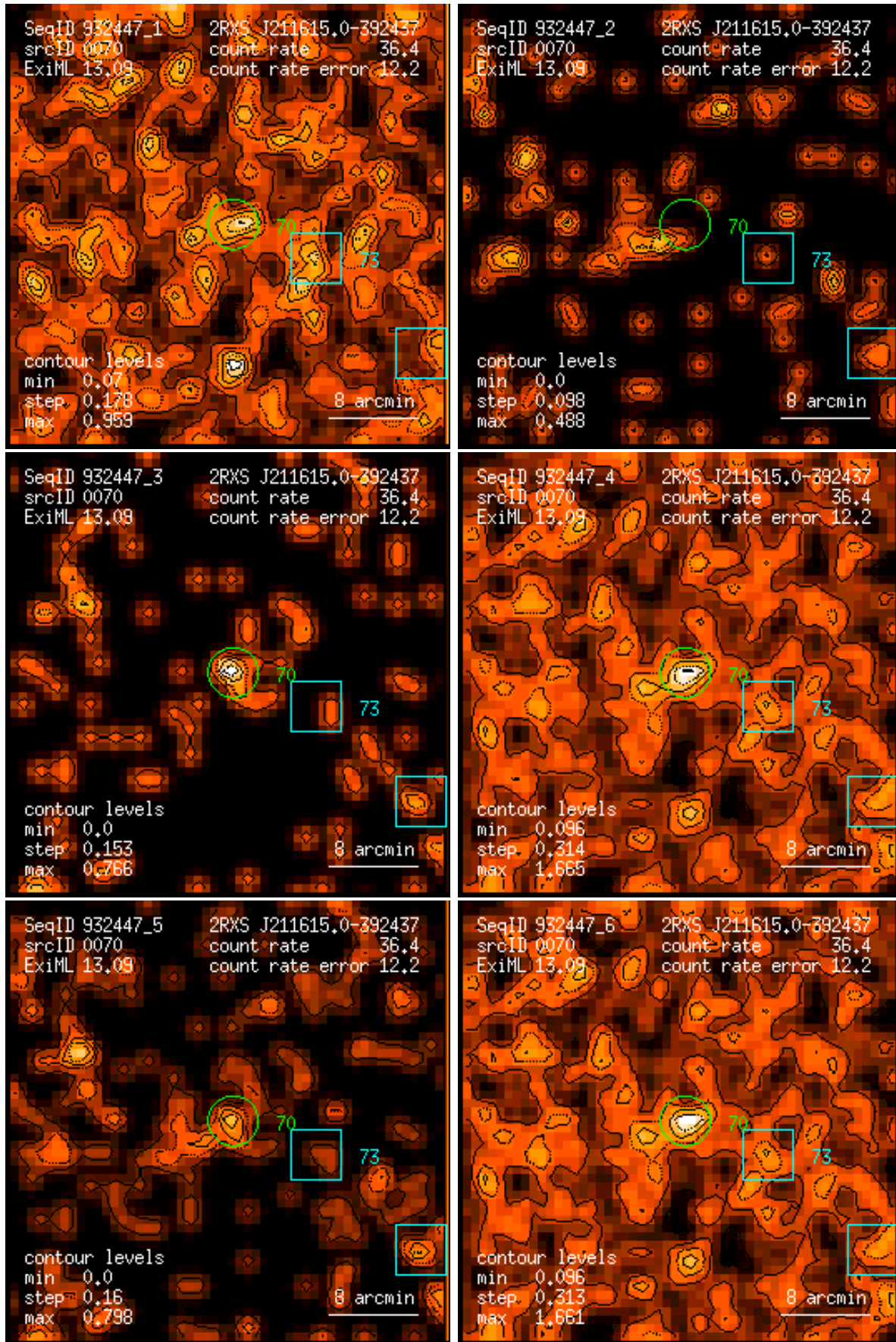
Figure 70: RASS 932447: detection 0070: band rate images, Gaussian filter: (1) PSPC channels 11 – 41, (2) 52 – 90, (3) 91 – 201, (4) 11 – 235, (5) 52 – 201, (6) 11 – 201. Broad band rates in counts/ks. Band rate contour levels in counts/ks/arcmin 2 .
