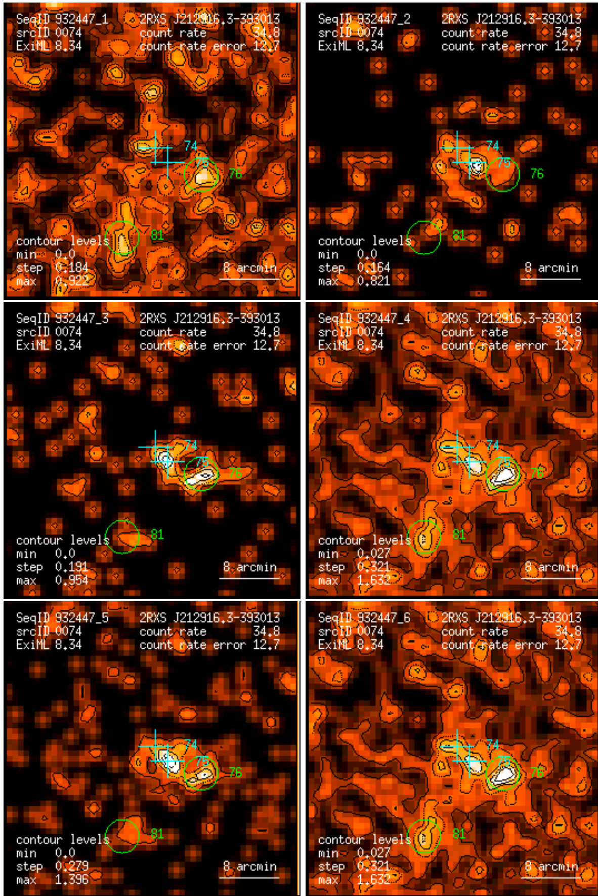
Figure 74: RASS 932447: detection 0074: band rate images, Gaussian filter: (1) PSPC channels 11 – 41, (2) 52 – 90, (3) 91 – 201, (4) 11 – 235, (5) 52 – 201, (6) 11 – 201. Broad band rates in counts/ks. Band rate contour levels in counts/ks/arcmin 2 .
